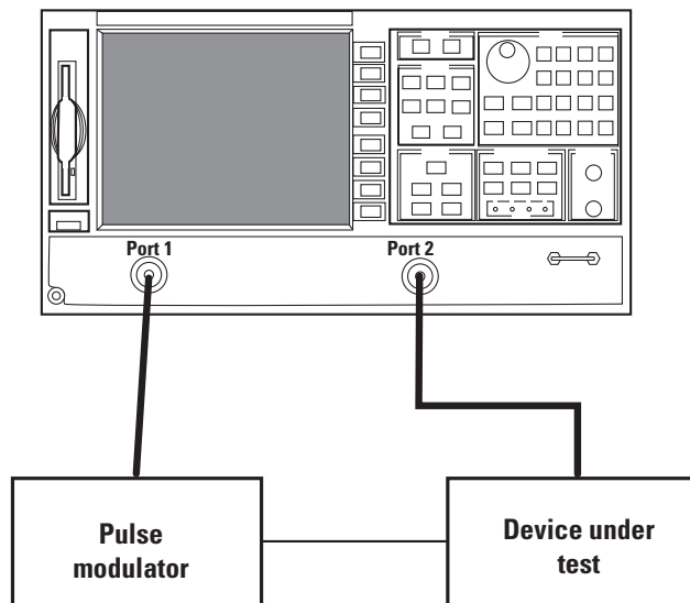
Figure 3. Simple transmission set up
