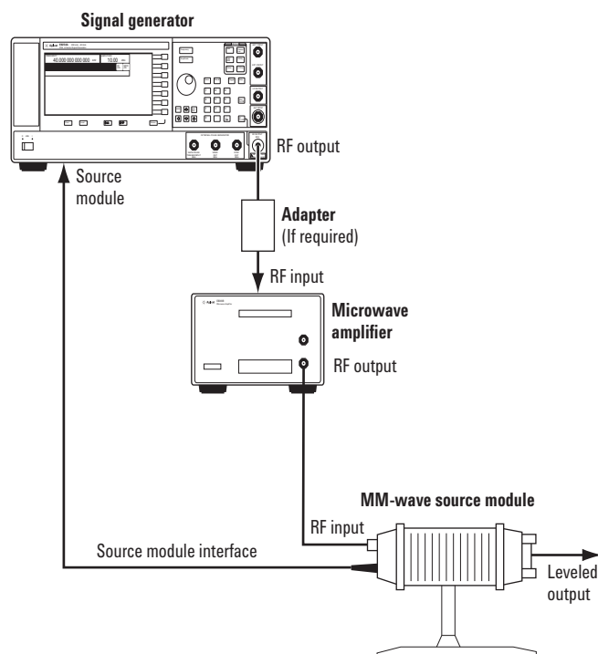
Figure 3-3. External Millimeter-wave source module leveling for a signal generator without Option 1EA.
