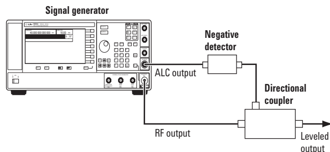
Figure 3-1. External detector leveling with a directional coupler.
