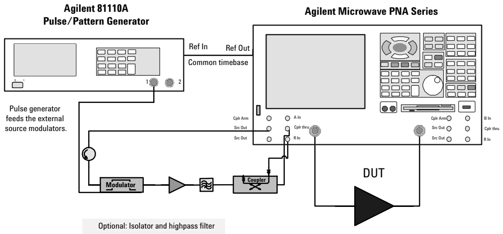
Figure 7. PNA Series pulsed setup.
