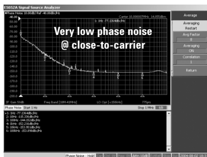
Figure 9. Crystal oscillator phase noise measurement by the E5052A SSA
