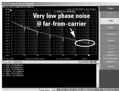
Figure 10. Free-running VCO phase noise measurement by the E5052A SSA
