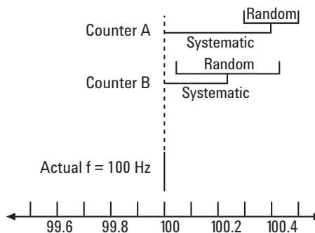
Figure 1. Simplified view of resolution vs. accuracy. Systematic errors related to the timebase “push” the displayed frequency away from the actual frequency. The random errors create a range of frequencies inside of which the counter can’t distinguish different signals.
