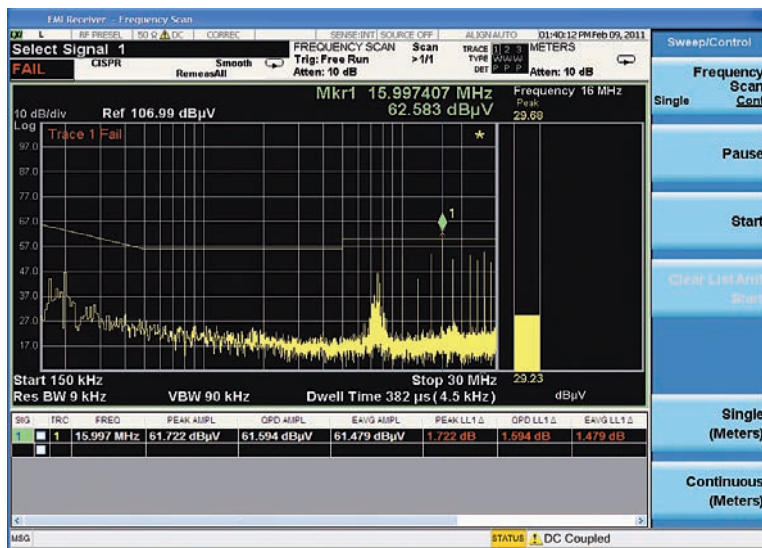
Figure 6. Conducted emissions failure QP measurement.
