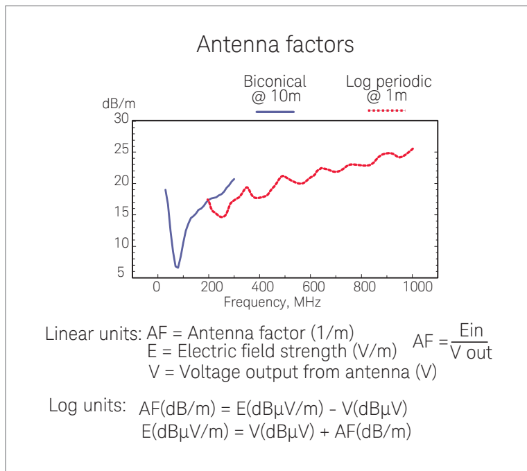
Figure B-1. Typical antenna factor shapes.
