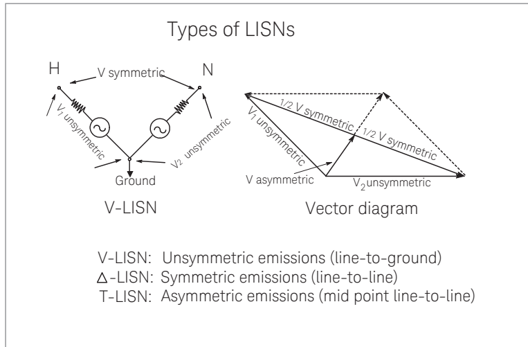
Figure A-2. Three different types of LISNs.
