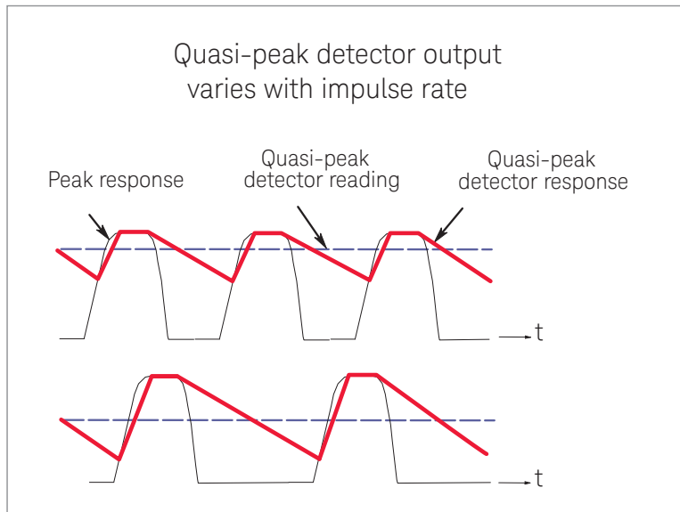
Figure D-2. Quasi-peak detector response diagram.
