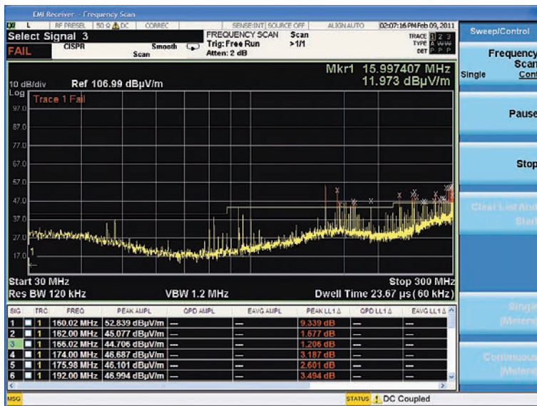
Figure 12. Ambient environment plus DUT emissions.
