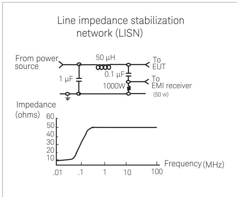
Figure A-1. Typical LISN circuit diagram.
