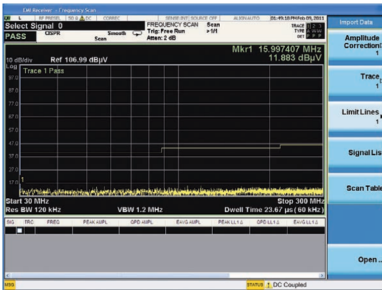
Figure 9. Loading FCC 3-meter Class B limit.
