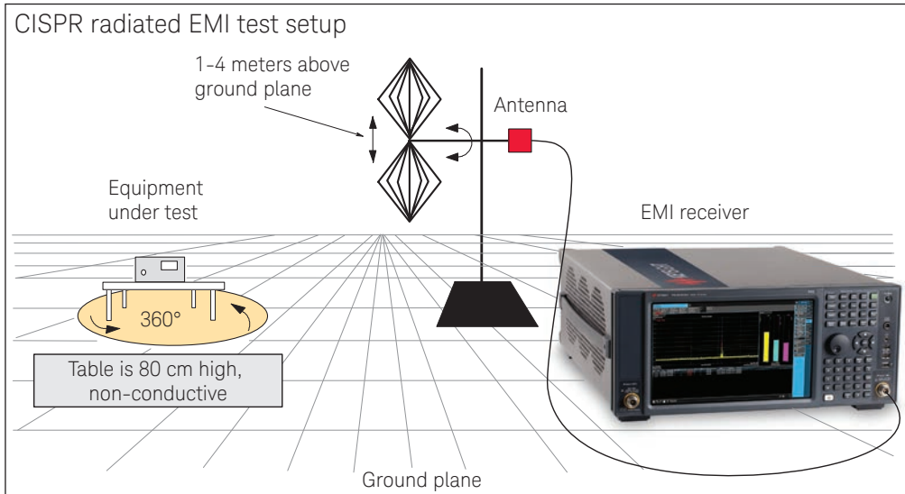
Figure 8. Radiated test setup.
