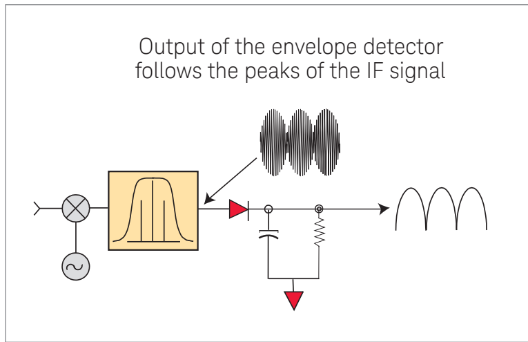
Figure D-1. Peak detector diagram.
