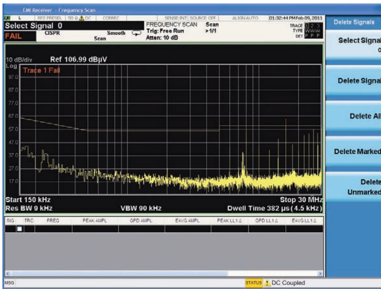
Figure 5. Conducted emissions from DUT.
