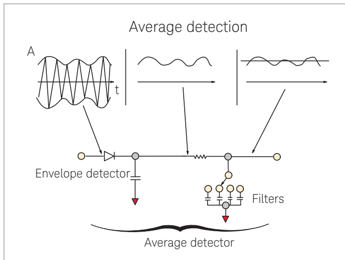
Figure D-3. Average detection response diagram.
