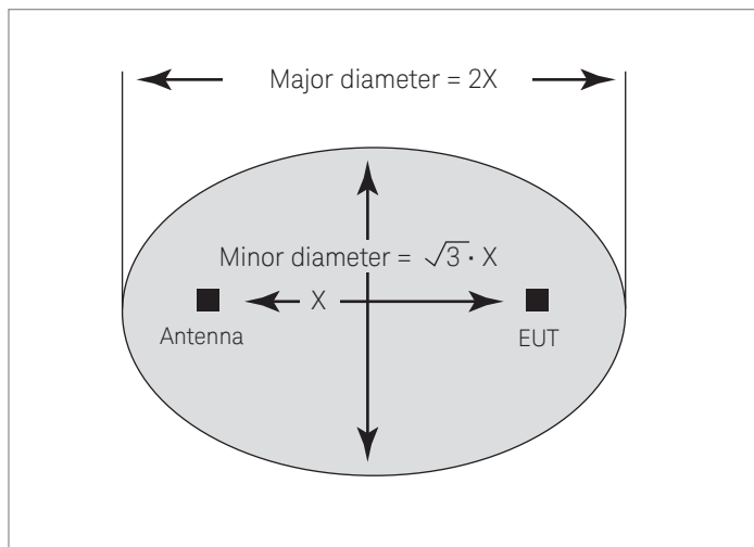
Figure 7. The CISPR ellipse.
