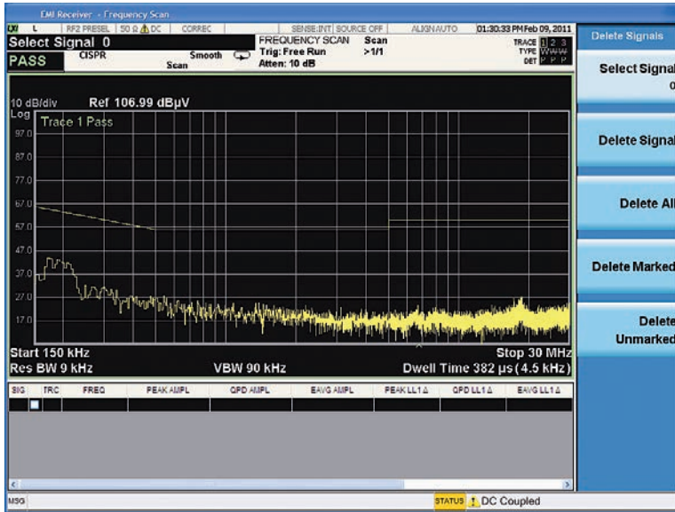
Figure 4. Test for ambient signals.
