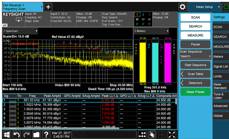
Figure 8. Scan and search for signals above the limit
