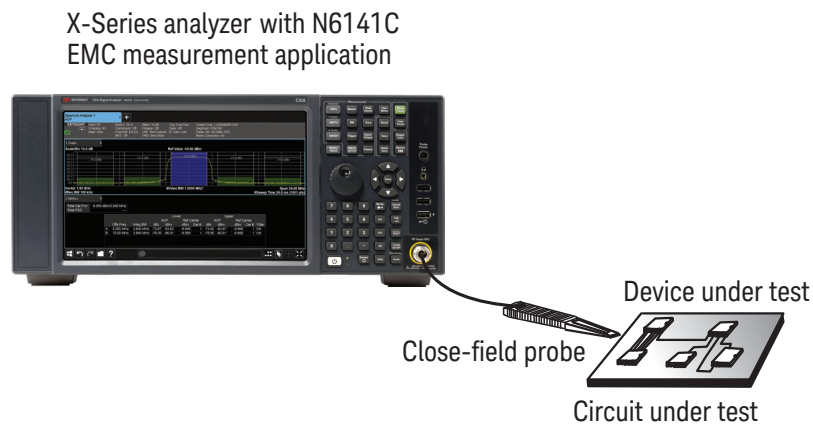
Figure 14. Diagnostics setup interconnection
