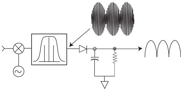
Figure D-1. Peak detector diagram
