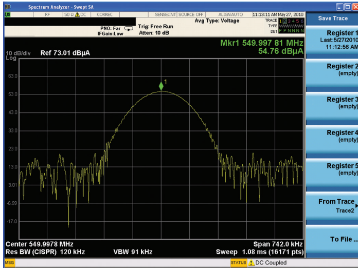
Figure 15. Preliminary diagnostics trace
