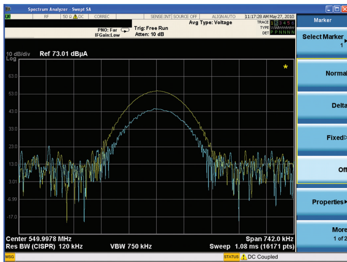
Figure 16. Diagnostics traces before and after redesign
