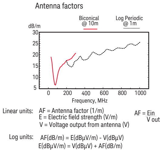
Figure B-1. Typical antenna factor shapes
