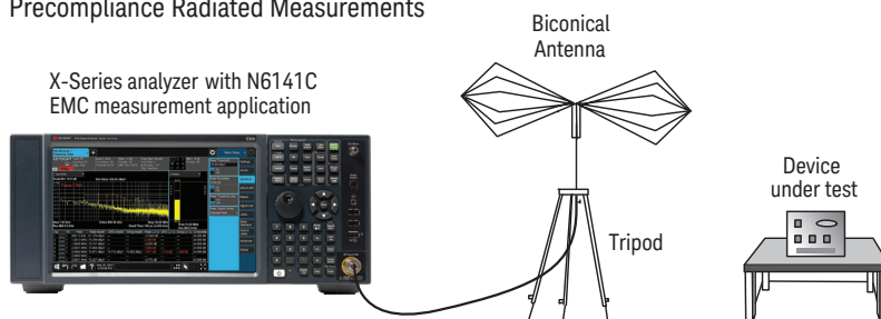
Figure 10. Radiated emissions test setup
