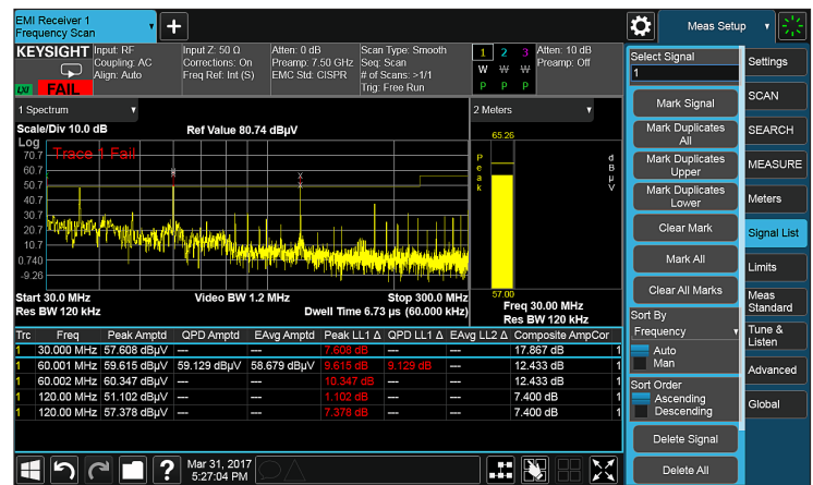
Figure 12. Duplicate ambient signals marked
