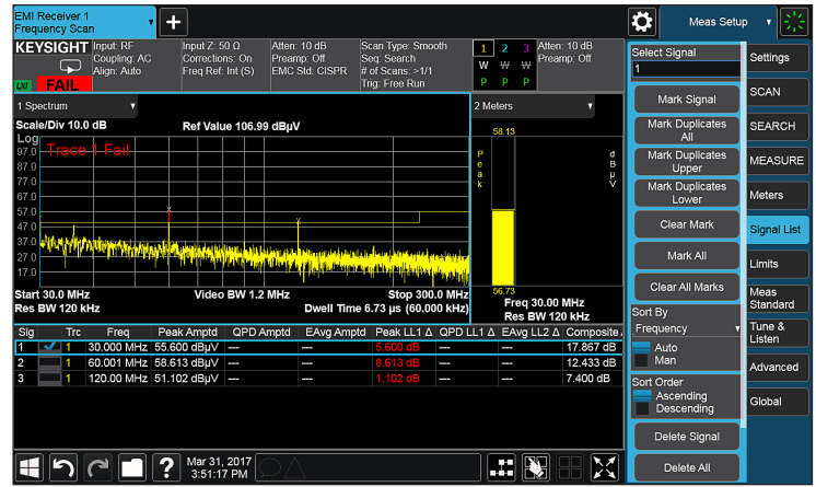
Figure 11. Mark ambient noise and delete it
