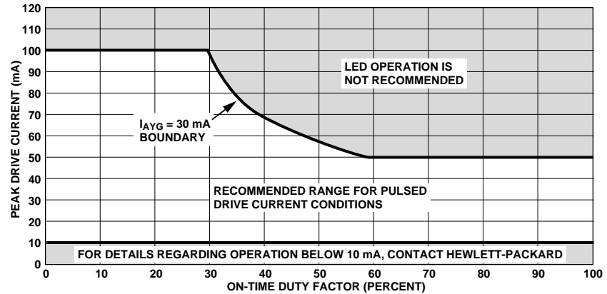
Figure 2. Recommended Range for Pulsed Drive Current Conditions for AllnGaP LEDs
