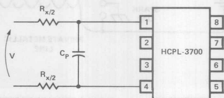
Figure 16. R_x C_p Transient Filter for the HCPL-3700
