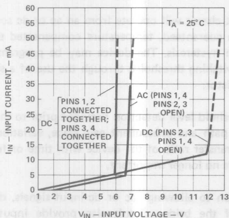
Figure 2. Typical Input Characteristics, I_{IN} vs. V_{IN}
