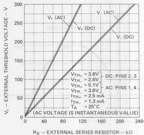
Figure 7. Typical External Threshold Characteristic, V_{\pm} vs. R_x
