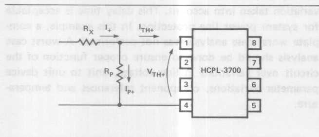
Figure 14. Threshold Accuracy Improvement through the Use of External R_x and R_p Resistors
