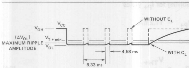
Figure 13. Output Waveforms of the HCPL-3700
