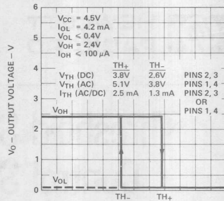
Figure 3. Typical Transfer Characteristics of the HCPL-3700
