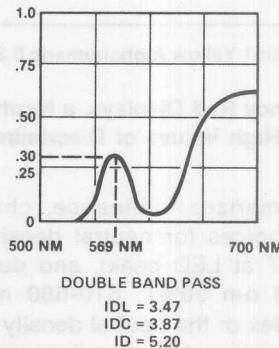
Figure 43. HDSP-2303 Green Alphanumeric 0.20-inch Display.
