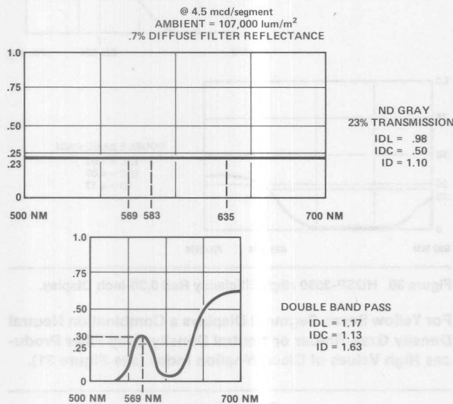
Figure 32. HDSP Green 0.30-inch Display.
