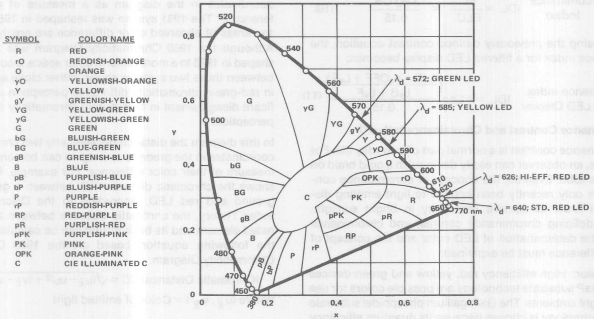
Figure 19. Dominant Wavelengths and Corresponding Colors for LEDs, Shown on the CIE Chromaticity Diagram.
