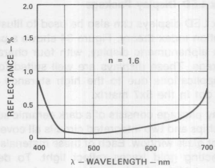
Figure 37. Front Surface Reflectance of Glass with Double Sided 1/4 Wave Optical Coating.
