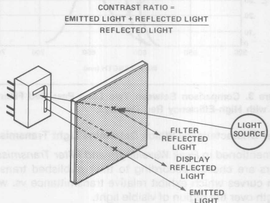
Figure 5. Luminance Contrast for a Light-Emitting Display with a Filter.
