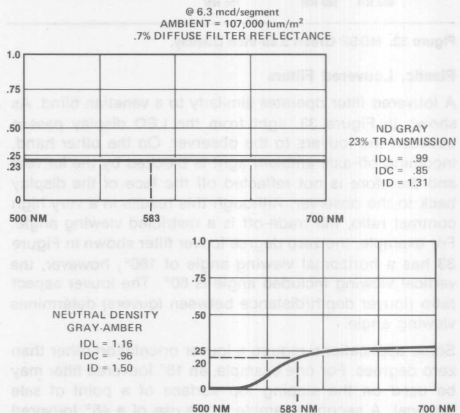
Figure 31. HDSP-4030 Yellow 0.30-inch Display.
