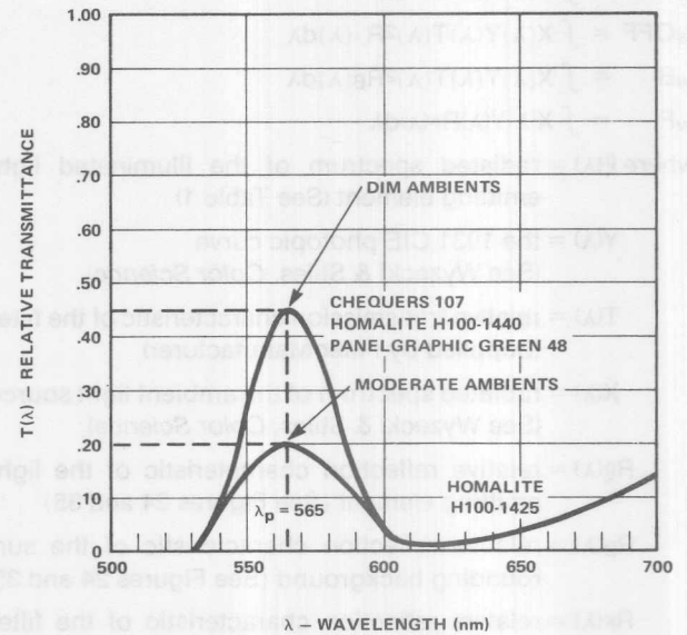
Figure 9. Typical Transmittance Curves for Filters to be Used with Green Displays.
