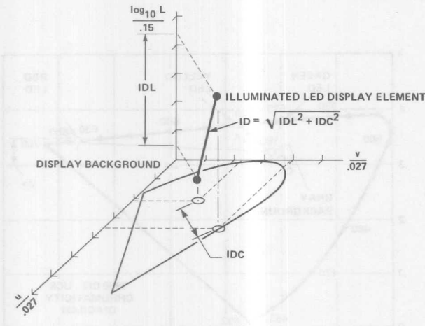
Figure 22. Photocolourimetric Space.
