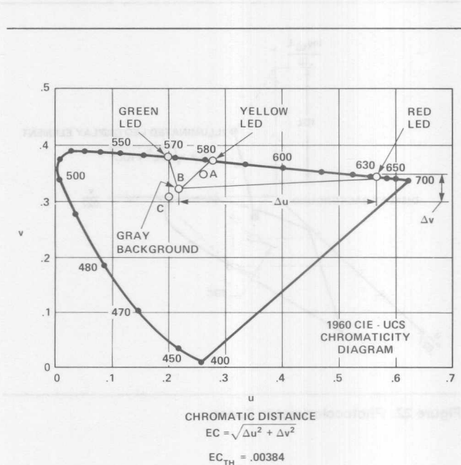
Figure 21. 1960 CIE-UCS Chromaticity Diagram with the Chromatic Distance Between a Green, Yellow or Red LED and a Gray Background.
