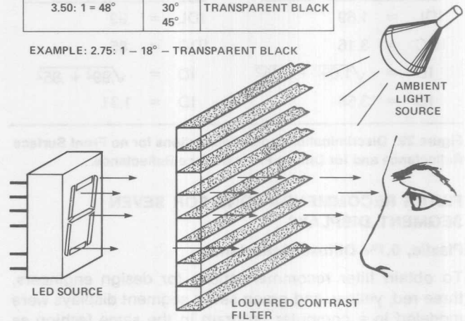
Figure 33. The Operation of a Louvered Filter.
