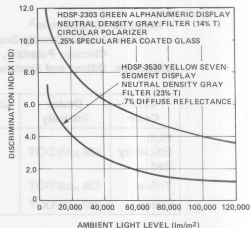
Figure 48. Effect of Reducing Ambient Lighting.
