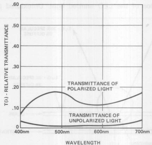
Figure 39. Spectral Characteristics of a Circular Polarizing Optically Coated Glass Filter.
