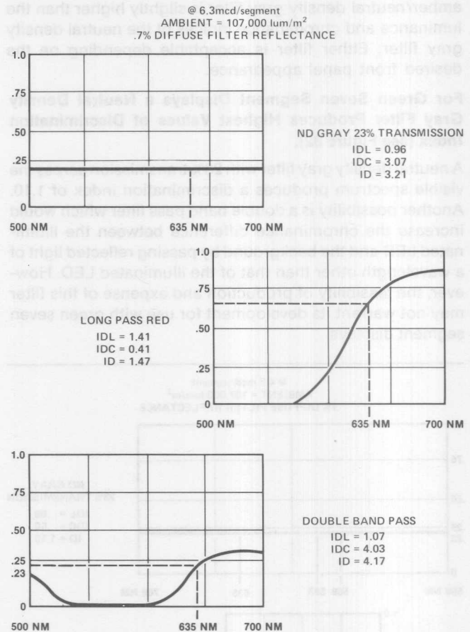
Figure 30. HDSP-3530 High Efficiency Red 0.30-inch Display.
