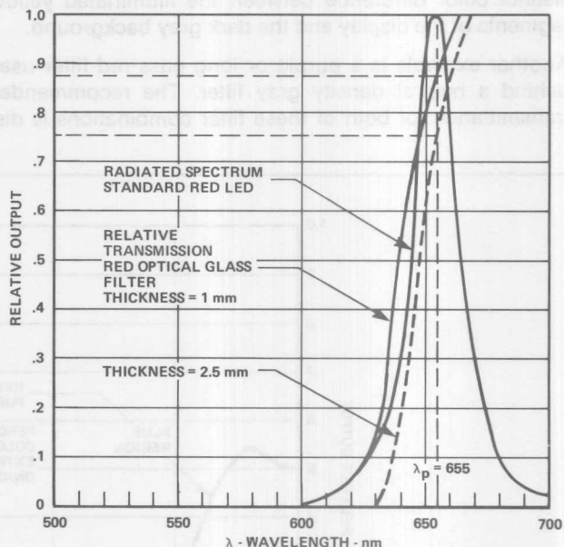
Figure 15. A Red Optical Glass Filter for use with High Efficiency Red LED Displays.
