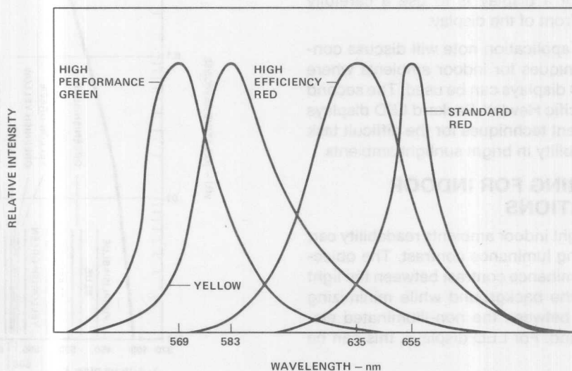
Figure 2. Relative Intensity vs. Wavelength.
