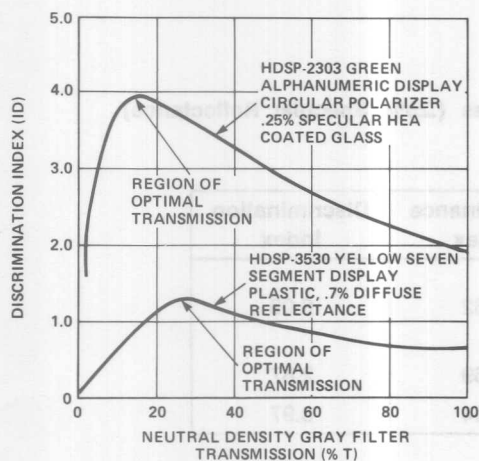
Figure 47. Optimal Neutral Density Gray Filter Transmission.
