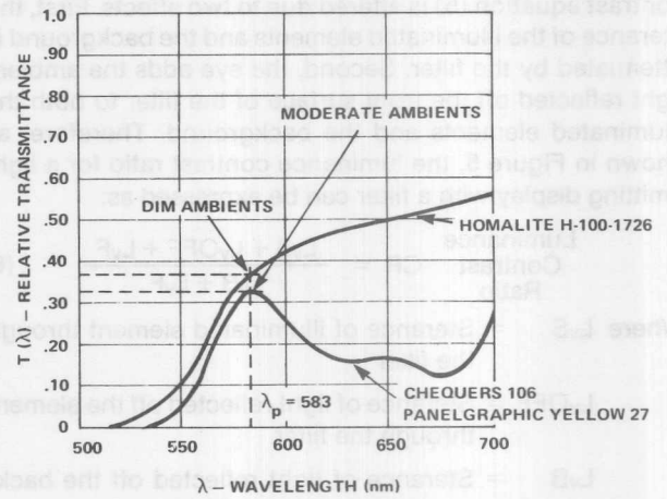
Figure 8. Typical Transmittance Curves for Filters to be Used with Yellow Displays.
