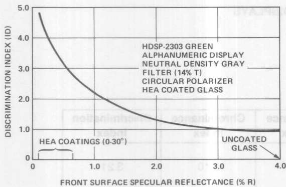
Figure 46. Effect of Reducing Front Surface Reflectance.
