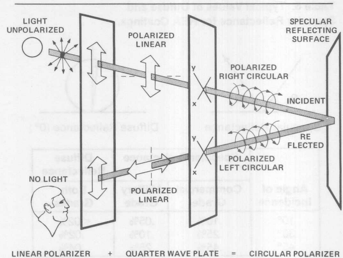
Figure 36. Operation of a Circular Polarizer.
