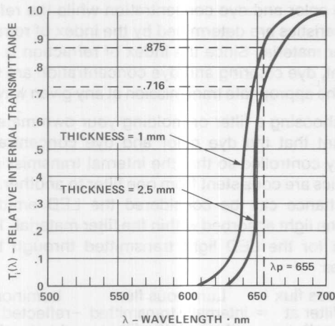
Figure 4. Variation in Relative Transmittance vs. Thickness for a Constant Density Filter Material.
