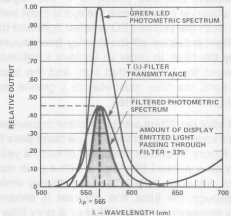
Figure 12. Effect of a Bandpass Wavelength Filter on a Green LED Display.
