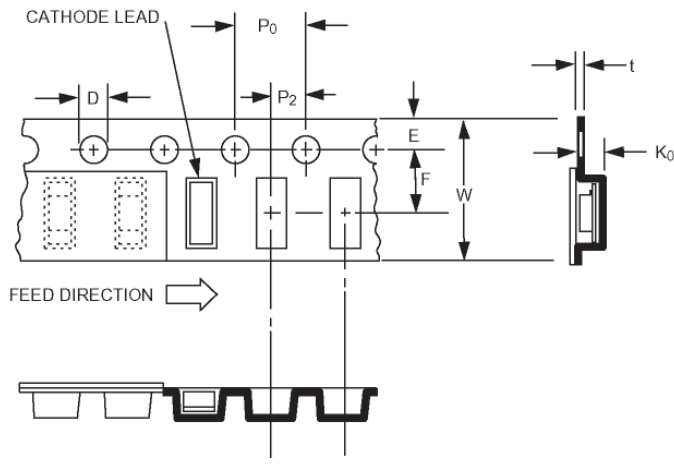
HSMX-H630 TAPE DETAIL
