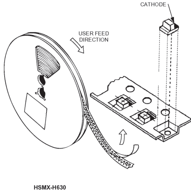
Figure 1c. 8 mm Embossed Cavity Carrier Tape Detail for HSMX-H630 and HSMX-H690, -S690 Chip LED Lamps.
