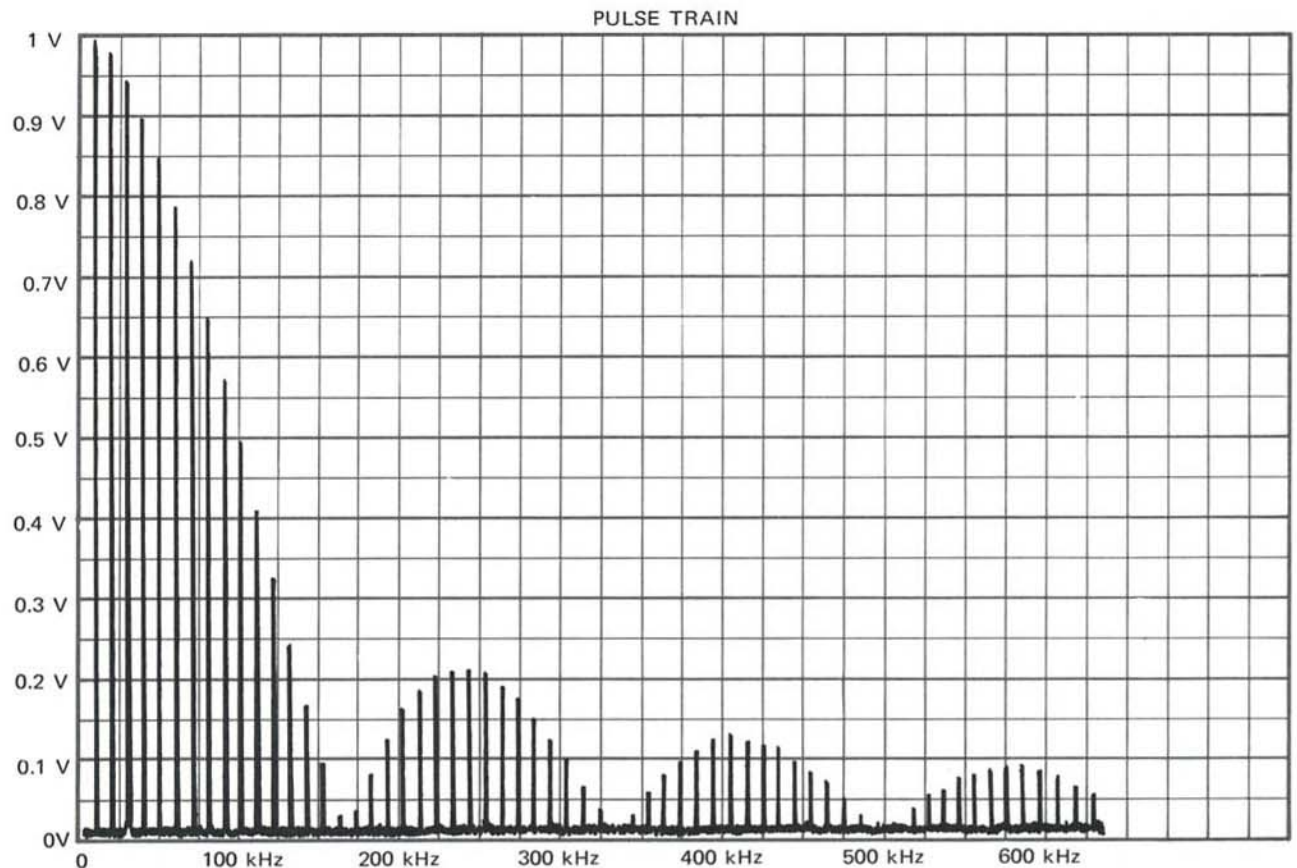
Figure 8 — Fourier analysis of pulse train.
