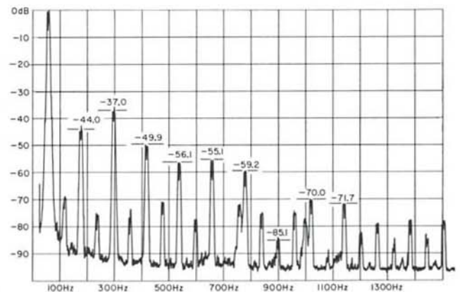
Figure 14 — Typical Power line distortion.
