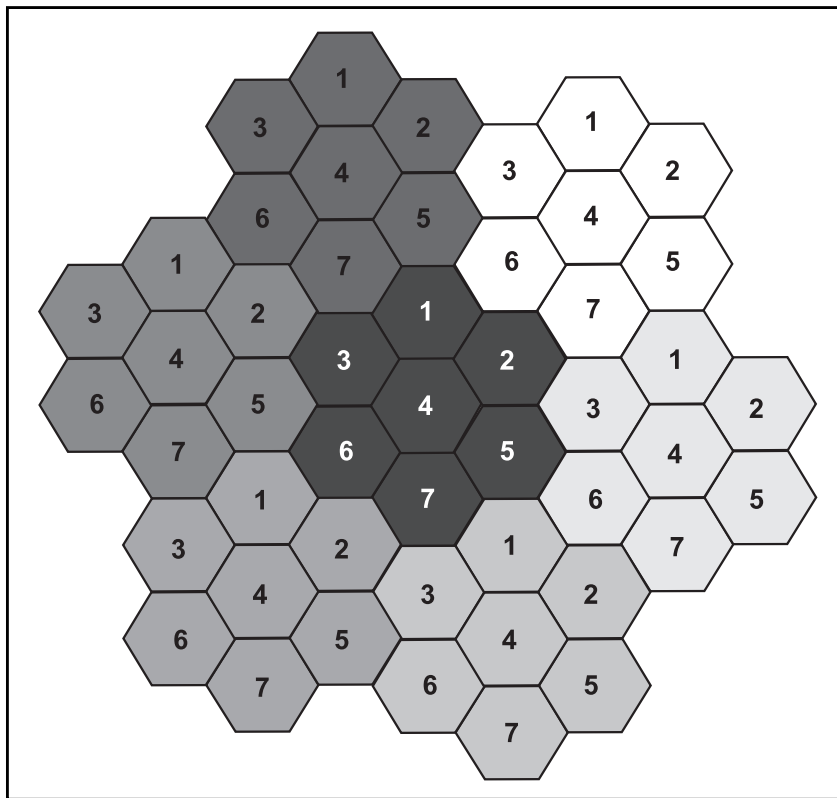
Figure 4. Cell clustering.
