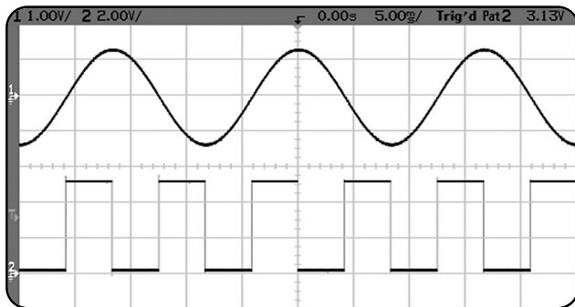
Figure 3: Falling edge of square aligned with max/min points of sine
