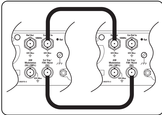
Figure 2: Two phase-locked 33120A generators. The generators are using a common clock signal and a common trigger signal.
