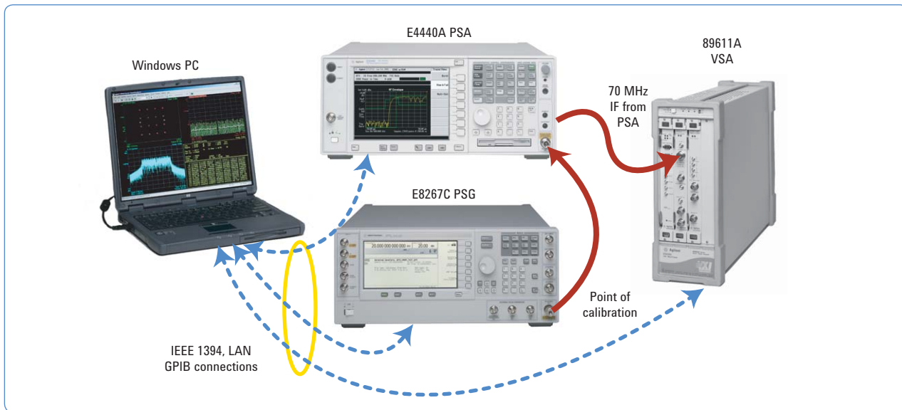
Figure 2. 89611A VSA with PSA (70 MHz IF out) calibration system, equipment setup example
