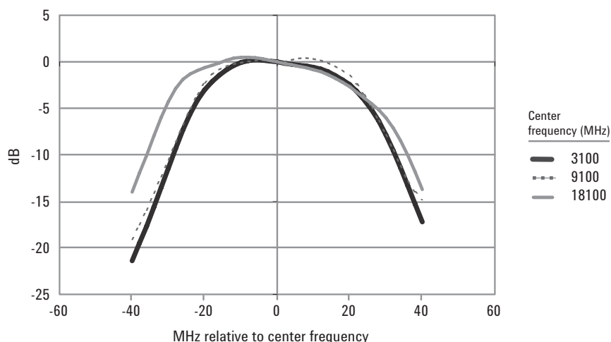
Figure 8. PSA Option 122 – 80 MHz IF response plotted by center frequency, without Option 123. For Option 140, the IF response is identical over –18 MHz to +18 MHz.
