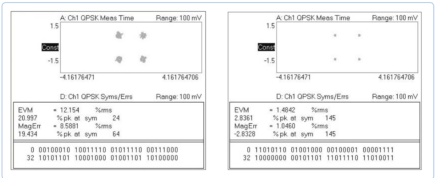
Figure 14. QPSK constellation and EVM summary table before (left image) and after (right image) extended calibration
