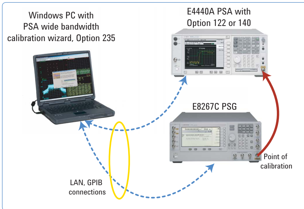
Figure 1. PSA Option 122 or 140 calibration system, equipment setup example
