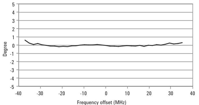
Figure 7. Phase deviation after calibration, 72 MHz span at 18.1 GHz (preselector bypassed)
