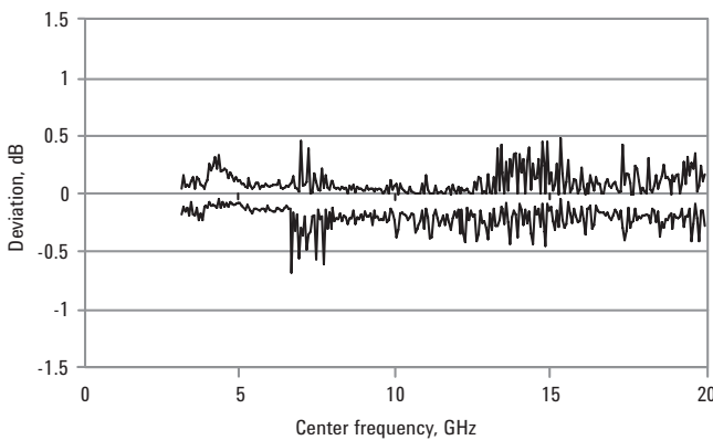
Figure 4. Nominal peak positive and negative amplitude deviation before calibration (preselector bypassed, 64 MHz bandwidth)
