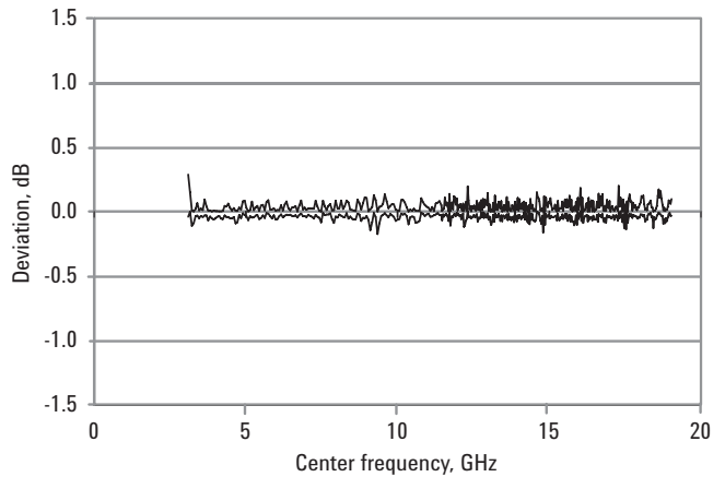
Figure 3. Nominal peak positive and negative amplitude deviation after calibration (using preselector, 64 MHz bandwidth)
