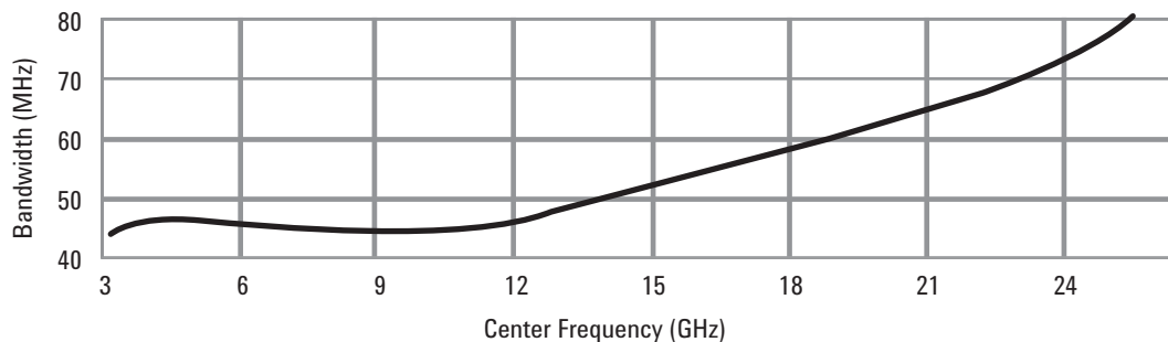
Figure 9. PSA Option 122 nominal IF bandwidth (–4 dB) versus center frequency, CF > 3.05 GHz, without Option 123. For Option 140, the IF response is identical over –18 MHz to +18 MHz.
