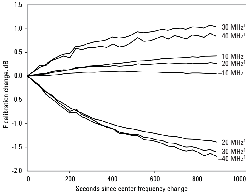
Figure 10. IF calibration change following a 19 GHz to 3.1 GHz center frequency change, for various offsets from center frequency (PSA Option 122)
