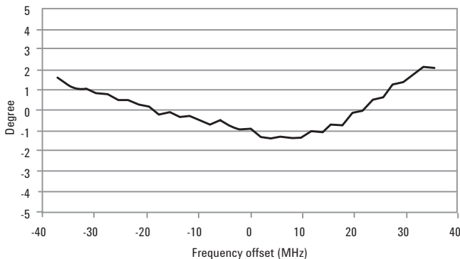
Figure 6. Phase deviation before calibration, 72 MHz span at 18.1 GHz (preselector bypassed)
