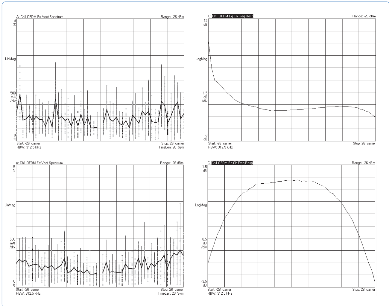
Figure 12. OFDM error vector spectrum and channel response before (top) and after (bottom) extended calibration 1
