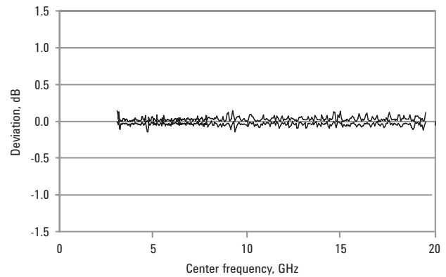
Figure 5. Nominal peak positive and negative amplitude deviation after calibration (preselector bypassed, 64 MHz bandwidth)
