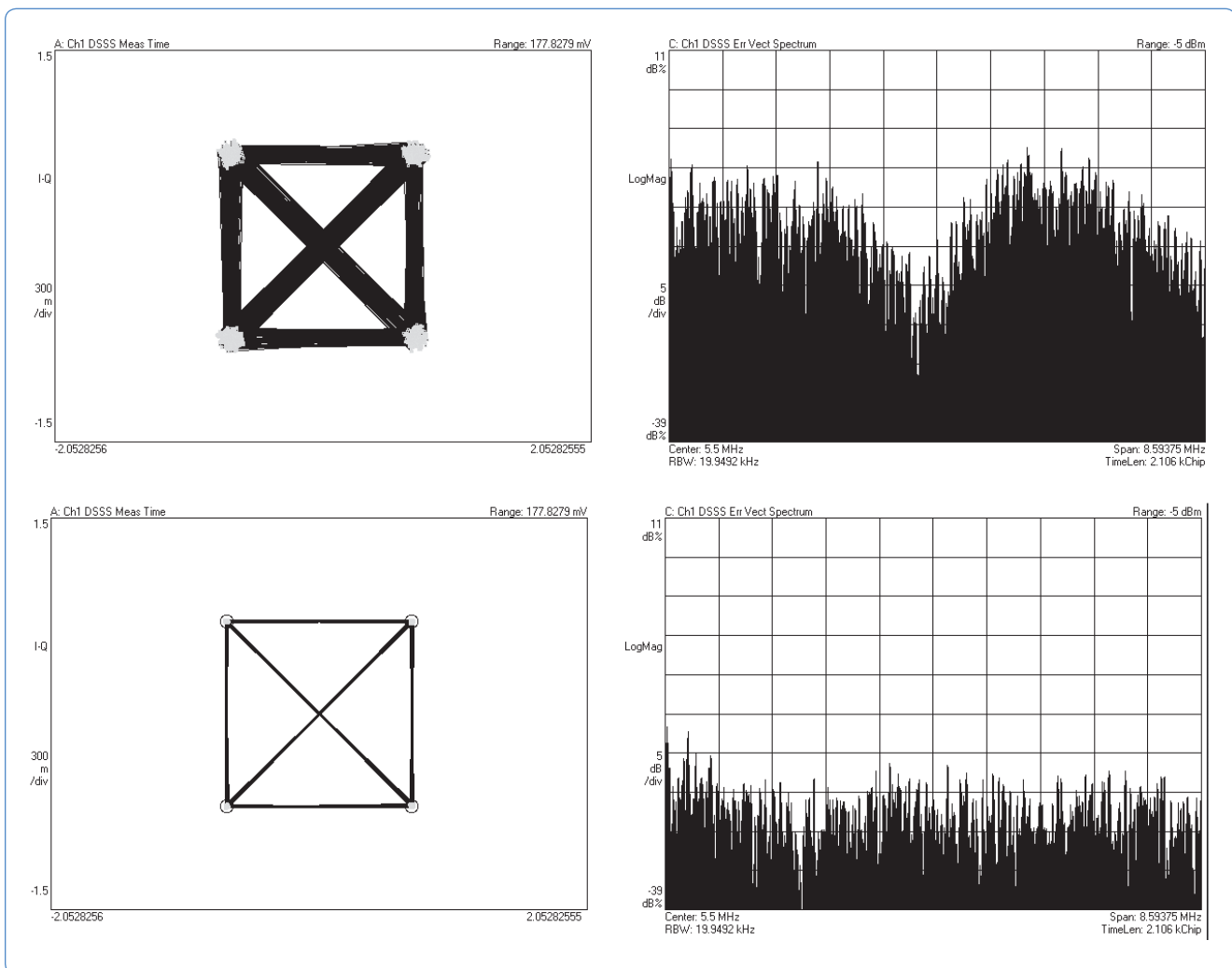
Figure 13. 802.11b error vector spectrum and constellation before (top) and after (bottom) extended calibration 1
