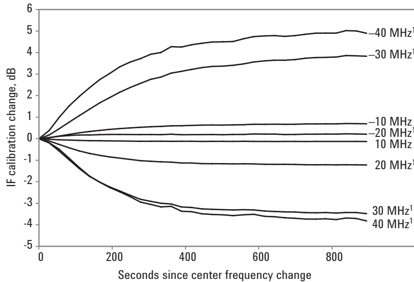
Figure 11. IF calibration change following a 3.1 GHz to 19 GHz center frequency change, for various offsets from center frequency (PSA Option 122)
