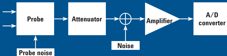
Figure 1. Noise sources
