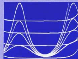
Figure 21. Equalizer peaking curve boost increments, at 100 Hz and 15 kHz center frequencies. Expanded scale 1 dB/vertical cm with calibration lines at 2 dB intervals log sweep, 20 Hz to 43 kHz.
