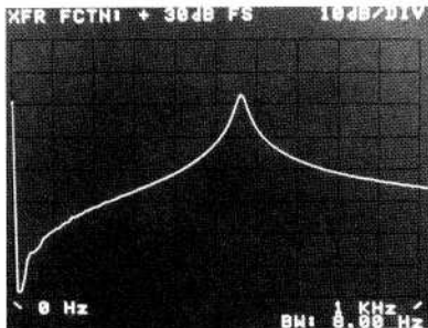
a) Frequency response magnitude
