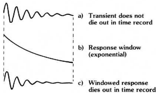
Figure 3.35 Using the response window
