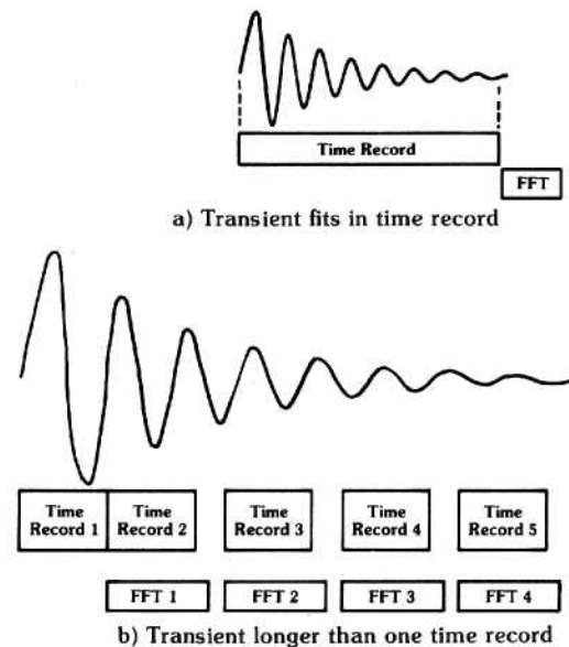
Figure 3.50 Transient analysis
