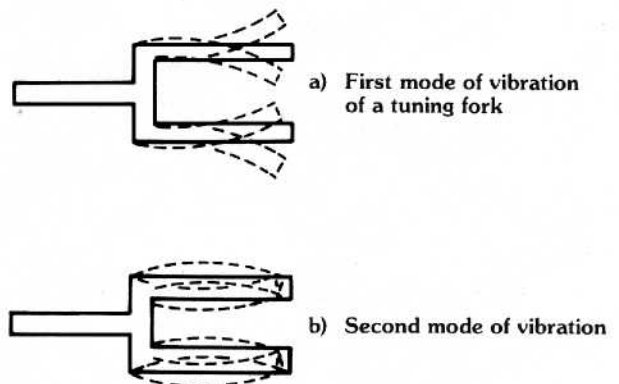
Figure 2.28 Example vibration modes of a tuning fork
