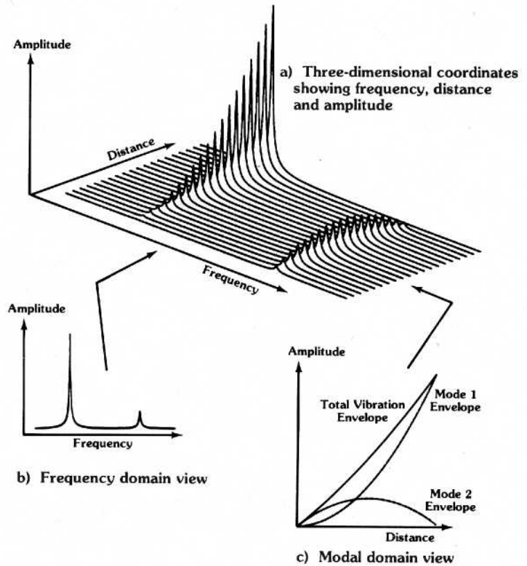
Figure 2.31 The relationship between the frequency and the modal domains
