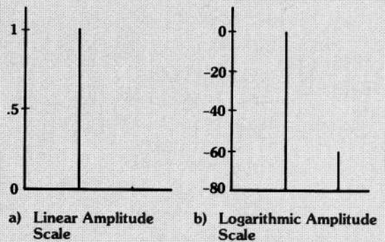
Figure 2.9 Small signals can be measured with a logarithmic amplitude scale.
