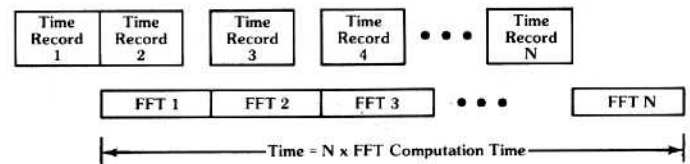
Figure 3.49 RMS averaging time
