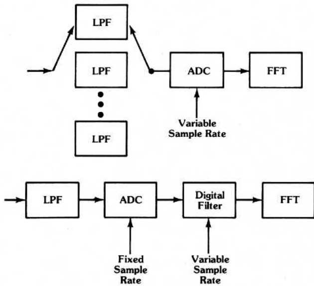
Figure 3.19 Block diagrams of analog and digital filtering
