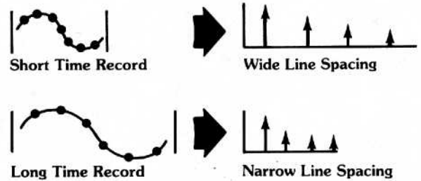
Figure 3.9 Frequency range of Dynamic Signal Analyzers is determined by sample rate
