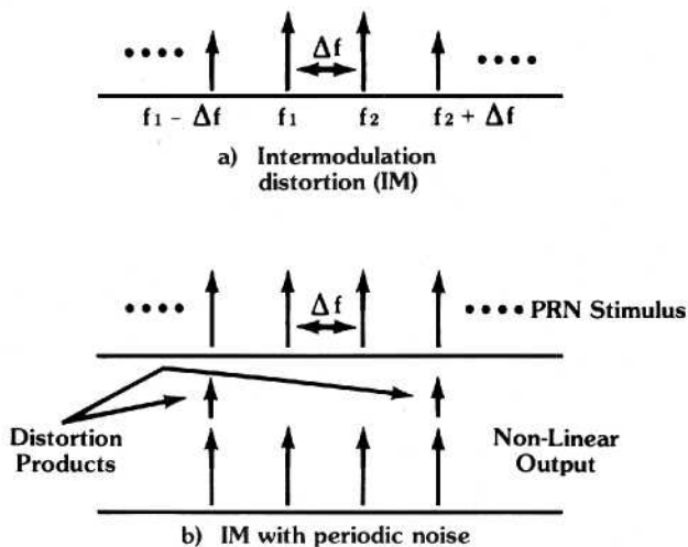
Figure 3.40 Pseudo-random noise distortion
