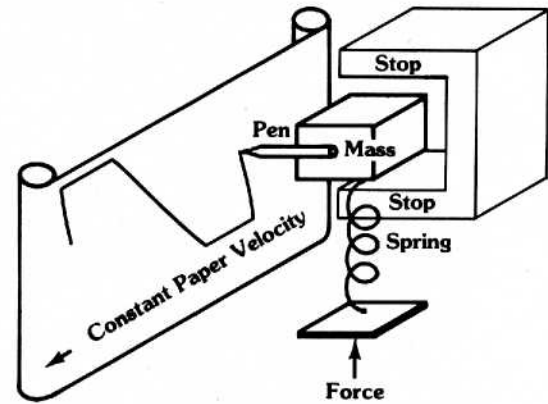
b) System is non-linear for large deflections
