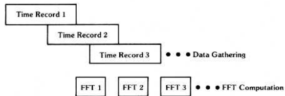
b) Overlapped processing is performed on data that combines old and new. The time between FFT's represents display processing.
