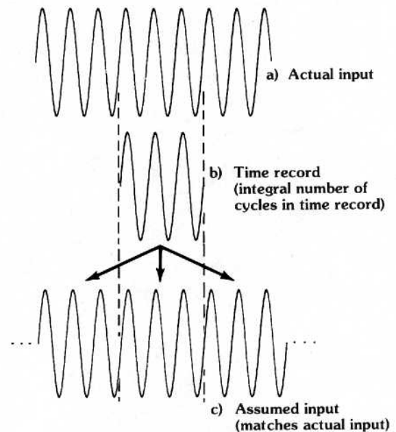
Figure 3.23 Input signal periodic in time record
