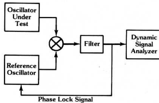
a) Block diagram of phase noise measurement
