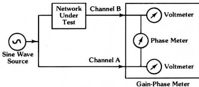
Figure 2.25 Gain-phase meter operation
