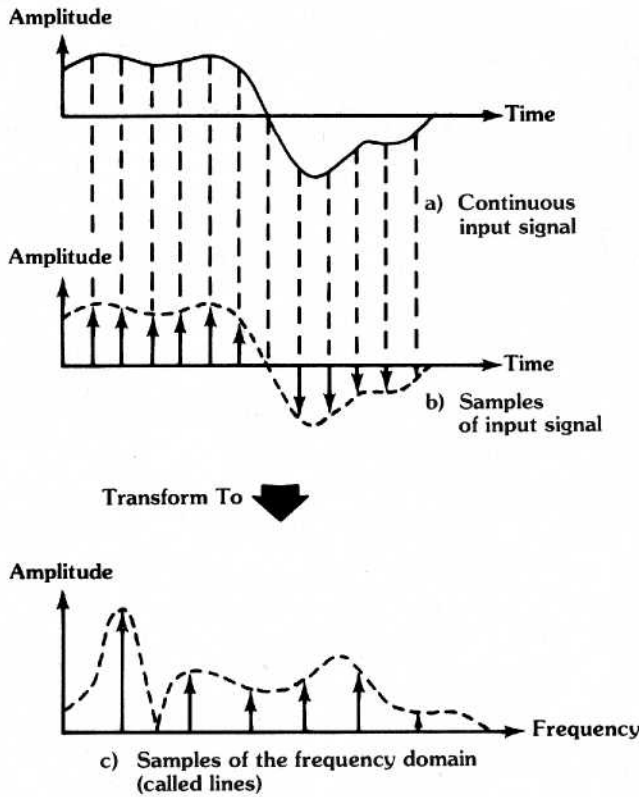
Figure 3.1 The FFT samples in both the time and frequency domains
