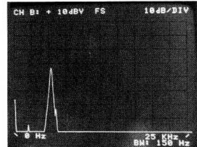
b) Hanning windowed transient
