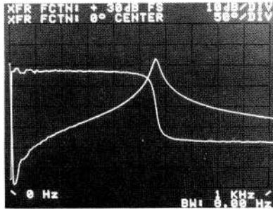
b) Frequency response magnitude and phase
