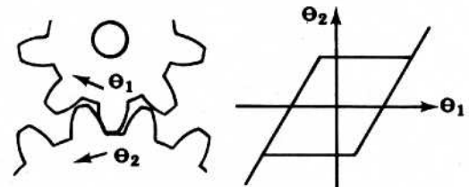
b) Backlash in a gear train
