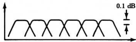
Figure 3.33 Flat-top passband shapes
