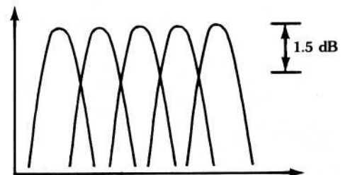
Figure 3.32 Hanning passband shapes
