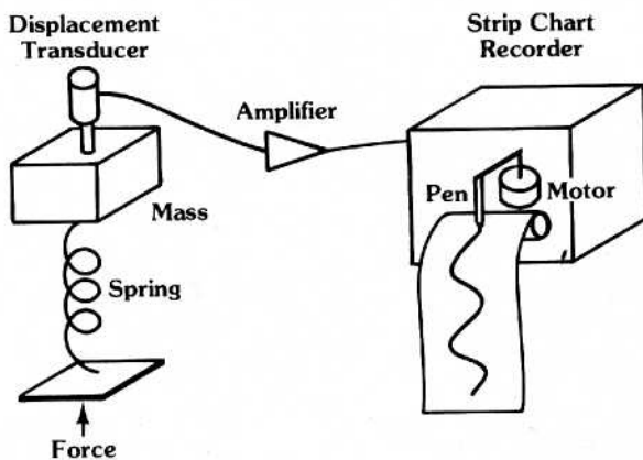
Figure 2.2 Indirect recording of displacement
