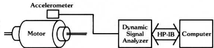
Figure 4.7 Desktop computer system for monitoring rotating machinery vibration
