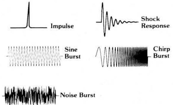
Figure 3.31 Self-windowing function examples
