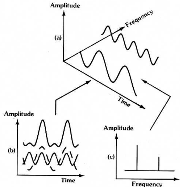
Figure 2.6 The relationship between the time and frequency domains.
