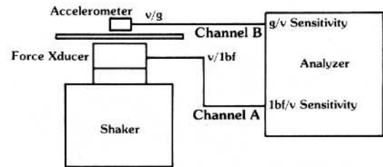
Figure 4.13 Engineering units set input sensitivities to properly scale results.
