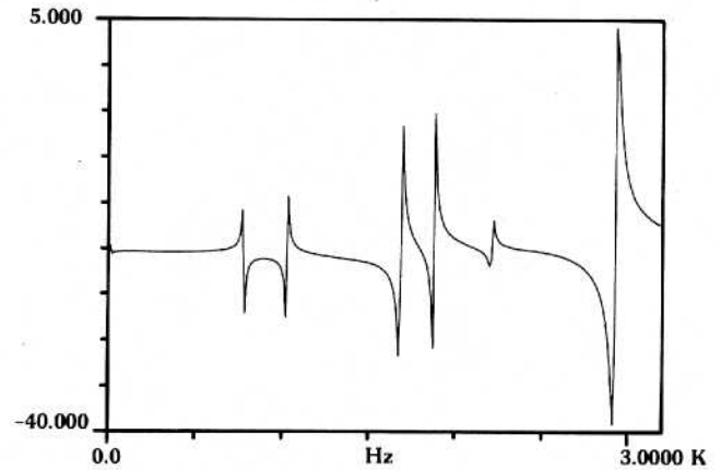
Figure 4.29 A frequency response of the plate.
