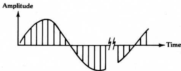
Figure 3.2 A time record is N equally spaced samples of the input
