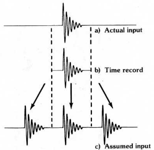
Figure 3.22 FFT assumption—time record repeated throughout all time
