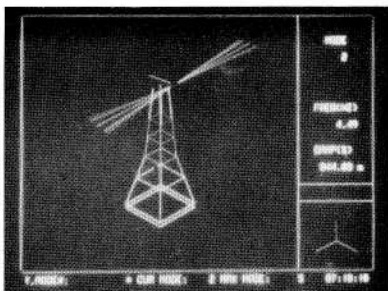
Figure 2.34 Measured mode shape
