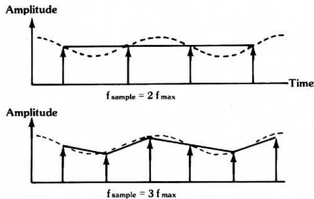
Figure 3.17 Nyquist criterion in the time domain
