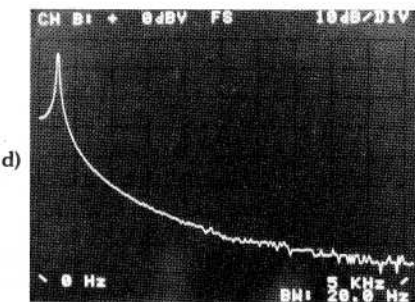
c) & d) Sine wave not periodic in time record
