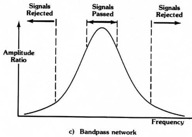
Figure 2.19 Three classes of frequency response
