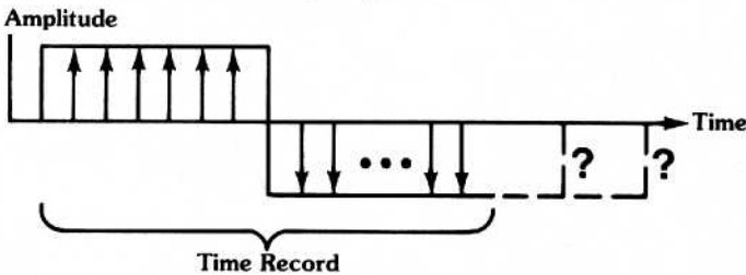
b) Period of input signal longer than the time record. Frequency of input signal is unknown.
