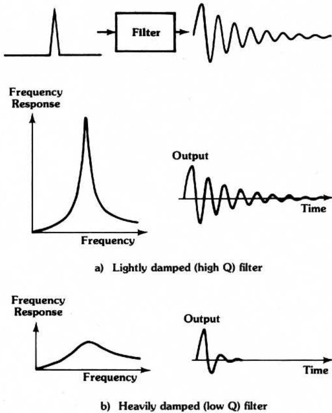
Figure 2.21 Time response of bandpass filters
