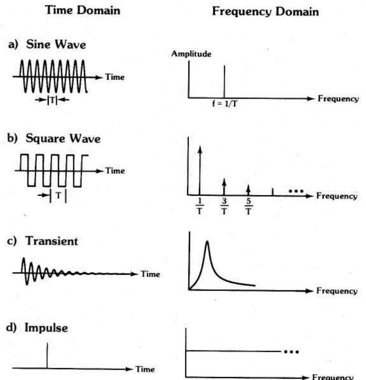
Figure 2.10 Frequency spectrum examples
