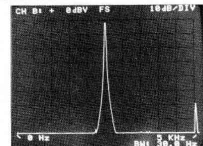
b) Windowed measurement — input not periodic in time record
