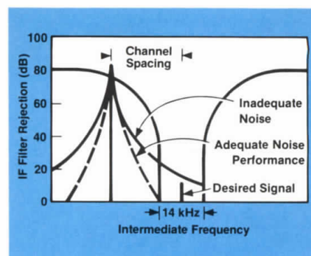
Figure 8.2. Signal generator phase noise in adjacent channel test.
