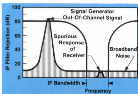
Figure 8.6. Broadband noise floor in spurious attenuation test.
