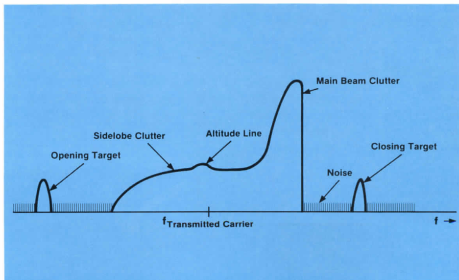
Figure 2.3. Typical return spectrum for airborne doppler radar.
