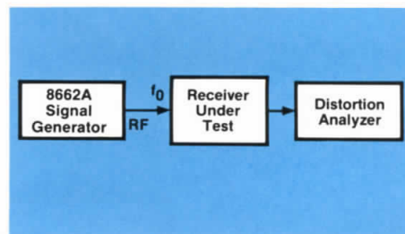
Figure 8.4. Receiver spurious attenuation measurement.
