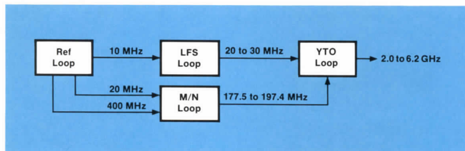
Figure 12.1. HP 8672A phase-lock loops.
