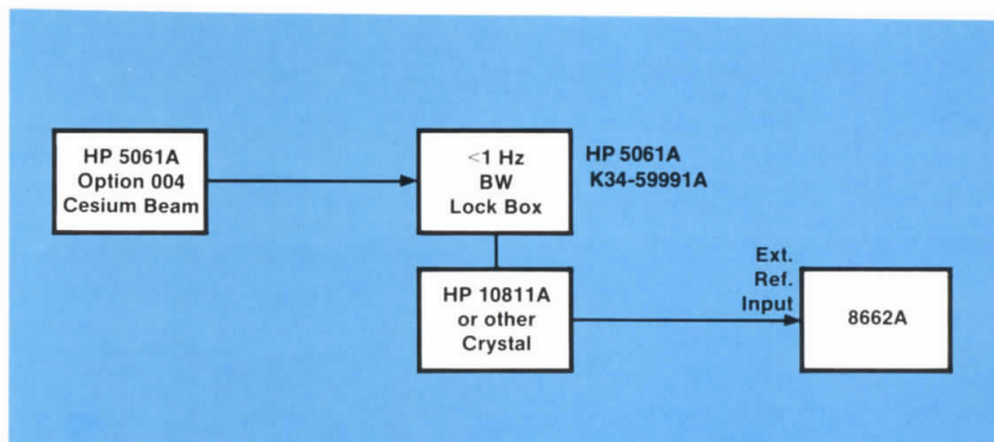
Figure 4.5. Using two references for optimal 8662A phase noise.
