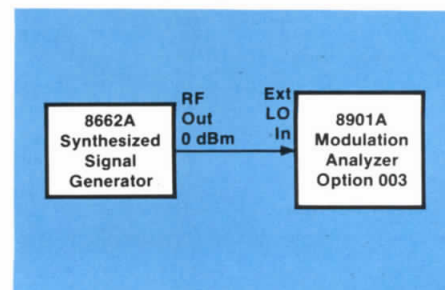
Figure 9.1. 8662A as external local oscillator for HP 8901A.
