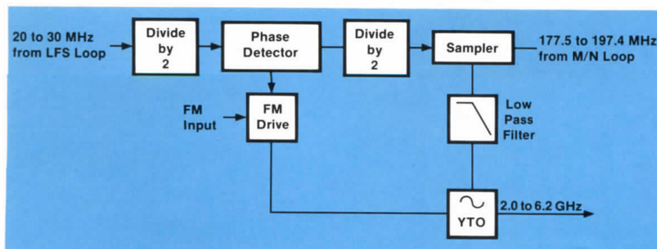
Figure 12.2. 8672A YTO loop.
