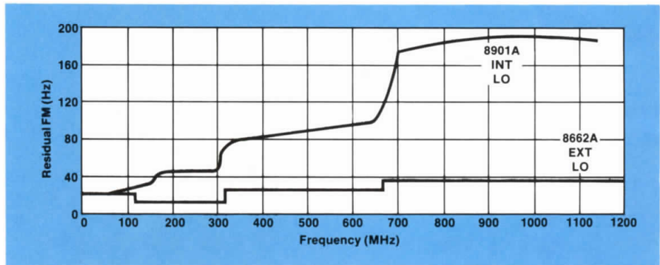
Figure 9.2. 8901A typical residual FM with no filtering.
