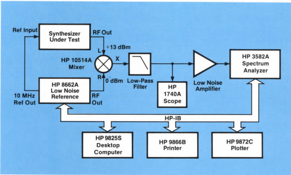
Figure 6.6. Automated system for phase noise measurement.
