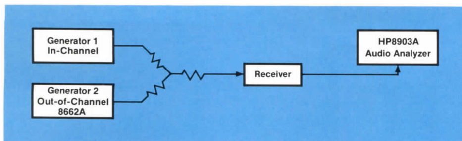
Figure 8.1. Receiver adjacent channel selectivity measurement.
