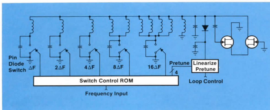
Figure 3.2. 320 to 640 MHz switched reactance oscillator.
