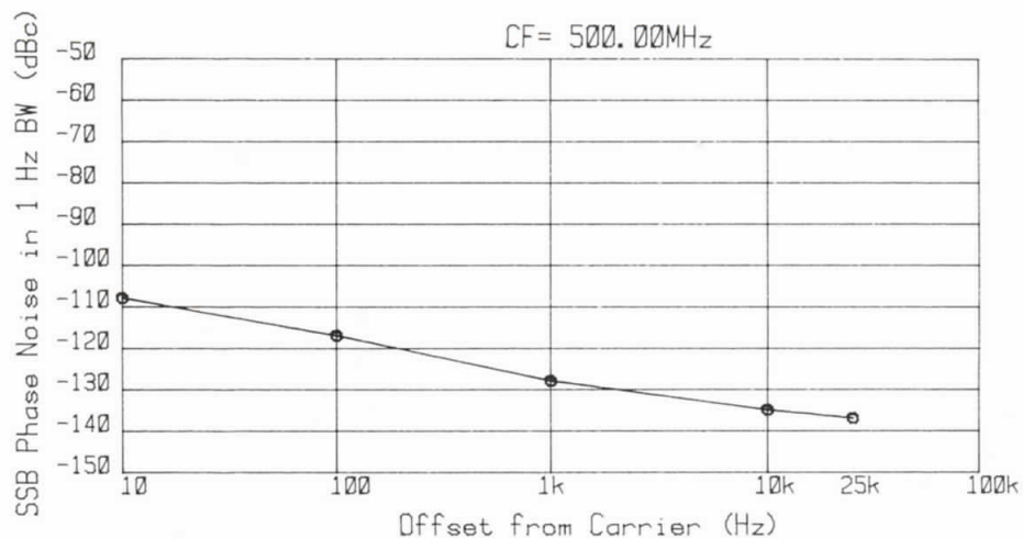
Figure 6.9. Typical hardcopy output from automatic measurement system.
