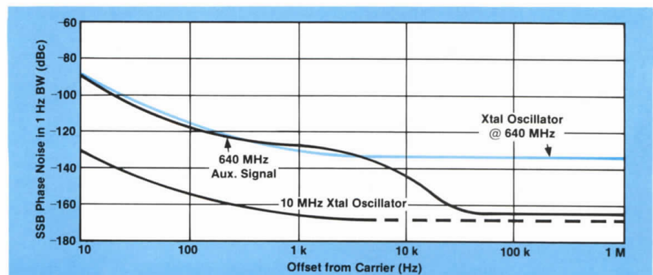
Figure 7.3. Phase noise of 640 MHz reference signal.
