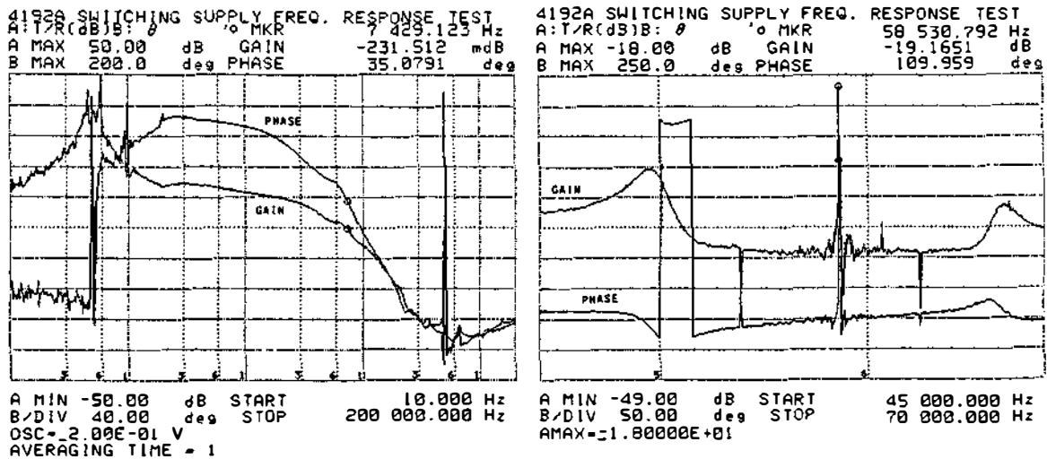
Frequency Response
