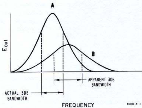
Figure 13. Curve A shows actual bandpass for gaussian IF amplifier. Curve B represents output when local oscillator frequency is swept too fast for IF amplifier to fully respond.
