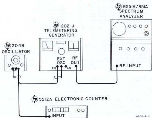
Figure 22. FM Deviation Measurement Using \text{hp} Spectrum Analyzer to Monitor Carrier Zero
