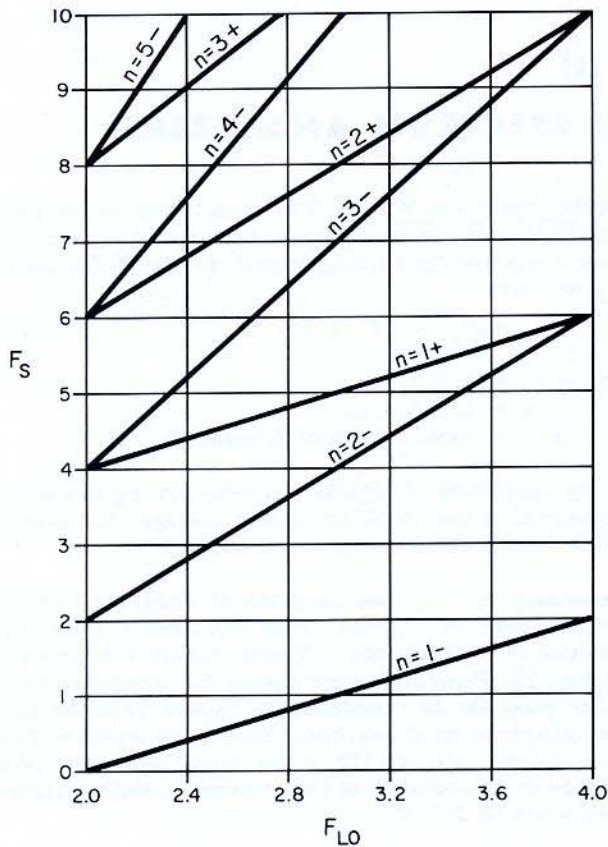
Figure 12a. Analyzer Tuning Curves for F_{if} = F_{lo}(\min) F_s = nF_{lo} \pm 2 \text{ gc}
