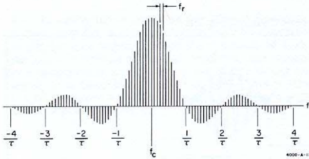
Figure 8. Resultant Spectrum of a Carrier Amplitude Modulated with a Rectangular Pulse
