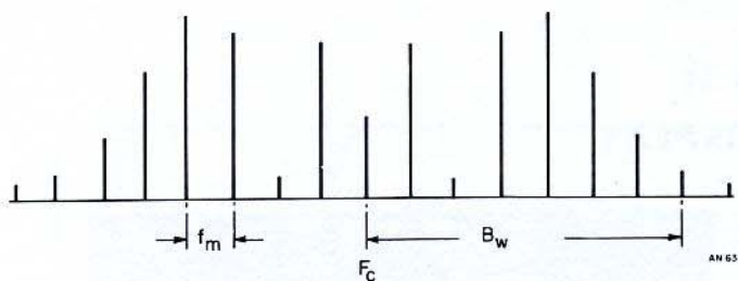
Figure 5. Amplitude Spectrum of Single Tone Frequency Modulation
