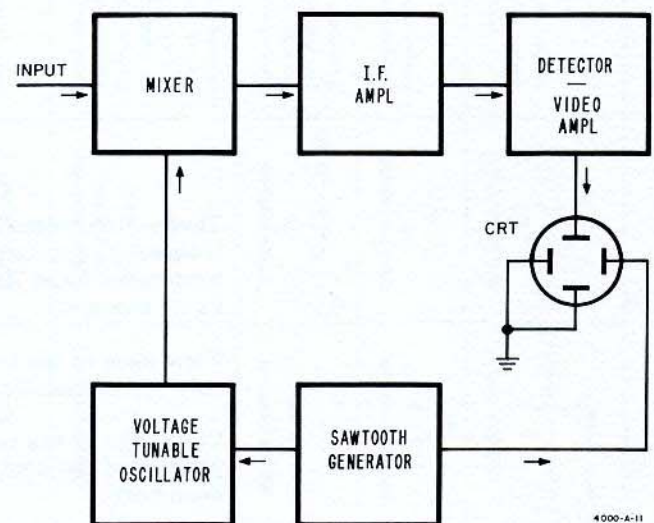
Figure 1. Simplified Spectrum Analyzer of the Swept-Receiver Design
