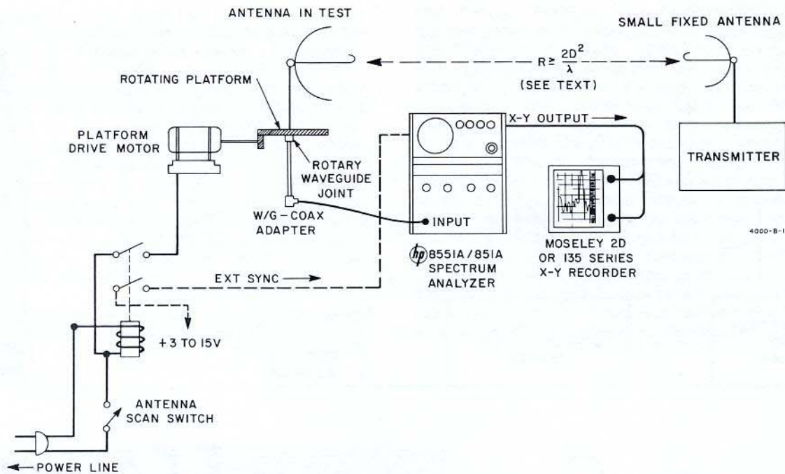
Figure 27. Spectrum Analyzer Connected for Rectilinear Antenna Pattern Plots
