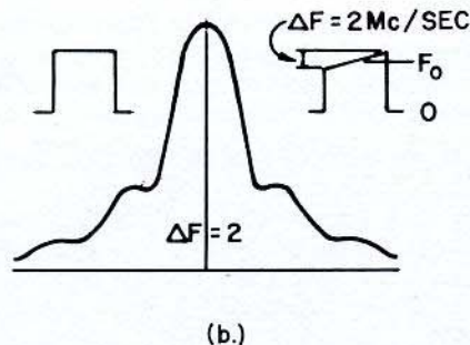
(b) Spectrum of rectangular pulse with linear FM resulting in increased sidelobe amplitude and minimas not reaching zero.
