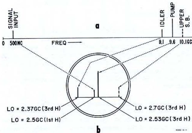
Figure 18. (a) Paramp Signals on a Linear Scale (b) Paramp Signals on Spectrum Analyzer Display
