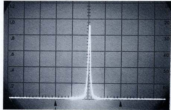
Figure 3. Spectrum of a CW Signal
