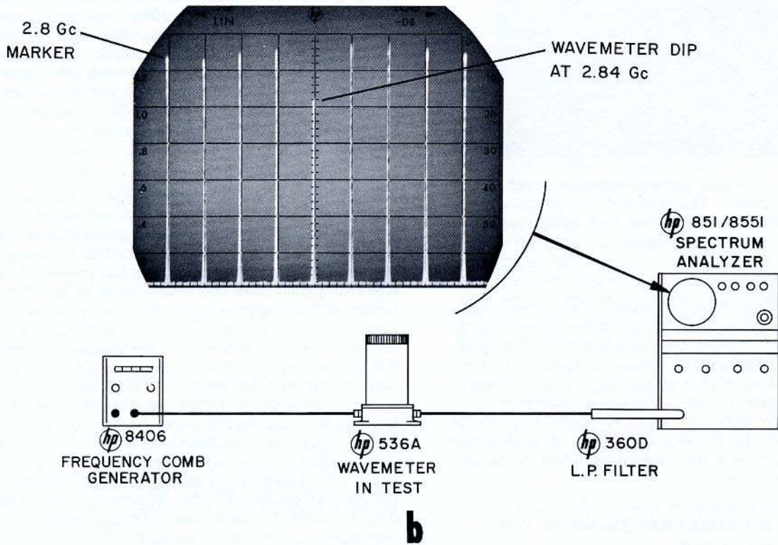
Figure 29. (a) Spectrum Analyzer and high accuracy Marker Generator setup for tuning transmitter frequency. (b) Spectrum Analyzer and Marker Generator setup for measuring frequency of passive device. A comb of frequencies may also be applied to an RF filter to display its bandpass characteristics.
