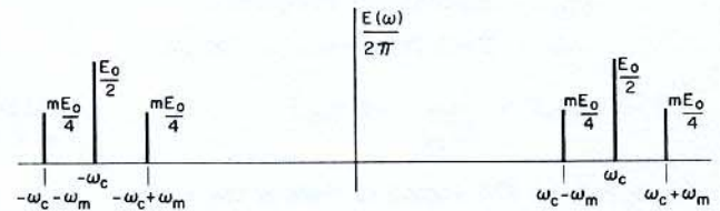
Figure A-1. Single Tone AM Spectrum
