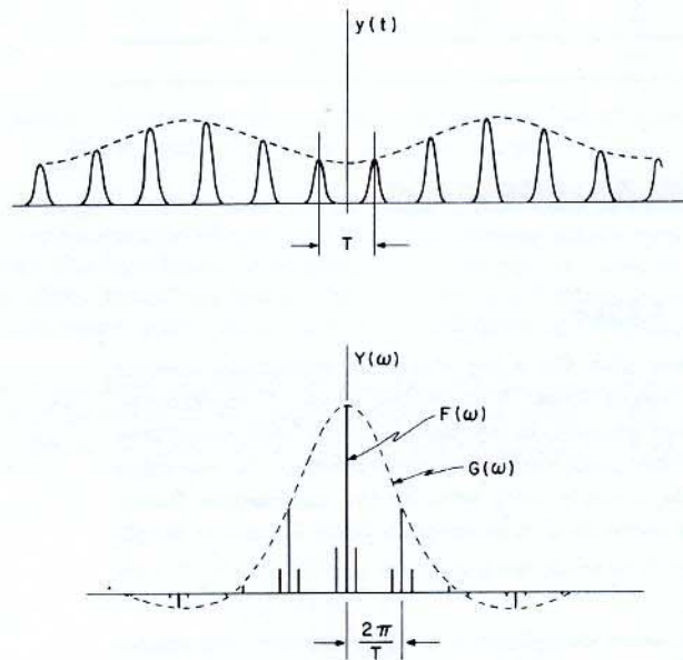
Figure A-4. Spectrum of an Amplitude-Modulated Pulse Train
