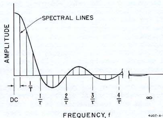
Figure 7. Spectrum of a perfectly rectangular pulse. Amplitudes and phases of an infinite number of harmonics are plotted resulting in smooth envelope as shown.
