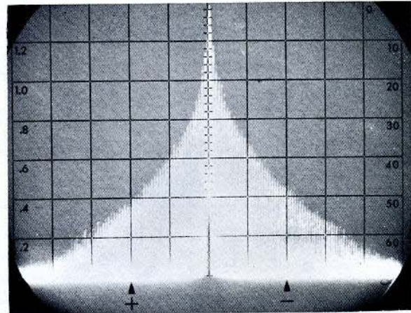
Figure 25. Spectrum Signature of a 0.5 \mu sec Pulse
