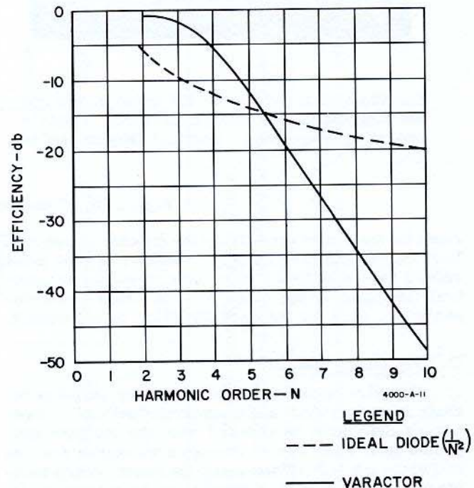
Figure 19. Comparison of Varactor and Rectifying Diode Harmonic Efficiency
