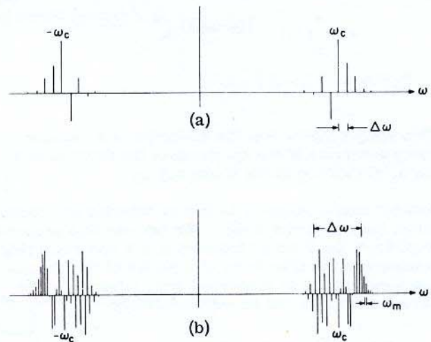
Figure A-3. Single Tone FM (a) M_f = 1 ; (b) M_f = 10
