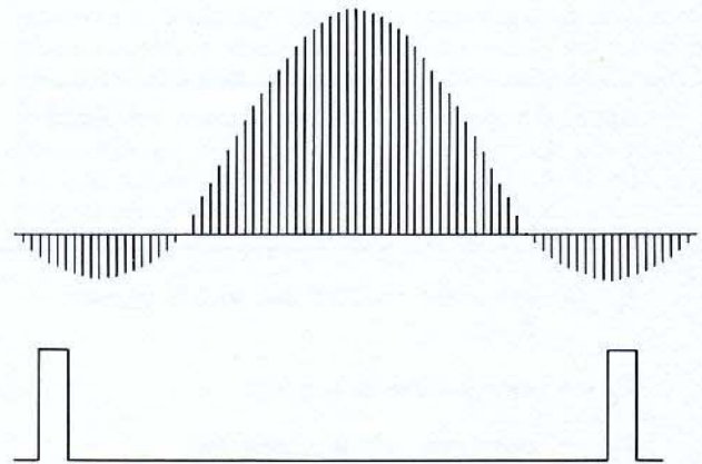
Figure 9c. PRF lower than 9a results in higher spectral density. Lobe width is same as a since pulse widths are identical.
