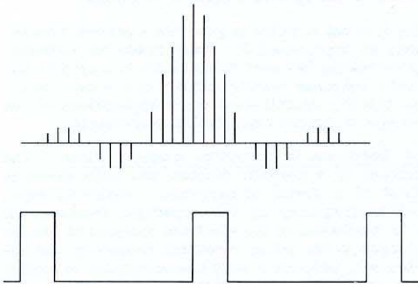
Figure 9b. Wider pulse than 9a causes narrower lobes but line density remains constant since PRF is unchanged.
