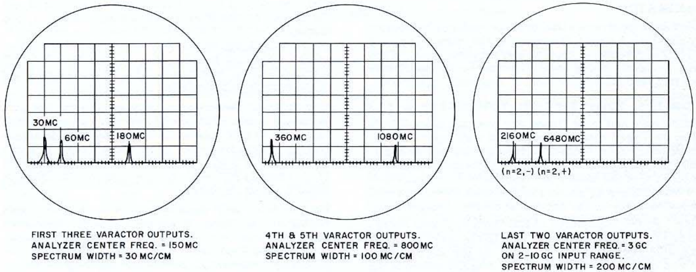
20 b. Analyzer Display Locations for Varactor Outputs
