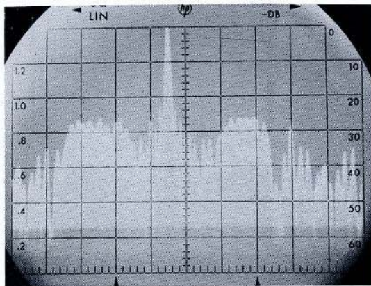
Figure 28. Antenna pattern obtained from Spectrum Analyzer. Vertical and horizontal outputs on rear panel also allow X-Y recording of display.
