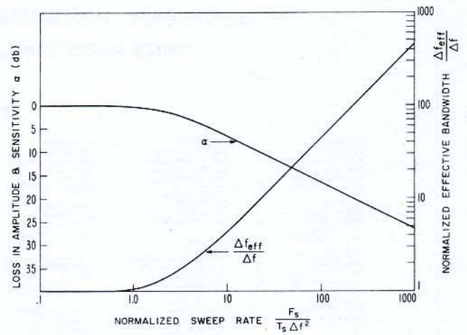
Figure B-2. Sensitivity Loss and Normalized Effective Bandwidth vs Normalized Sweep Rate
