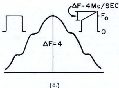
(c) Same pulse spectrum as (b) with more severe FM
