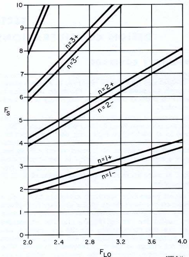
Figure 12b. Analyzer Tuning Curves for F_{if} = \frac{F_{lo}(\min)}{10} F_s = nF_{lo} \pm 200 \text{ mc}
