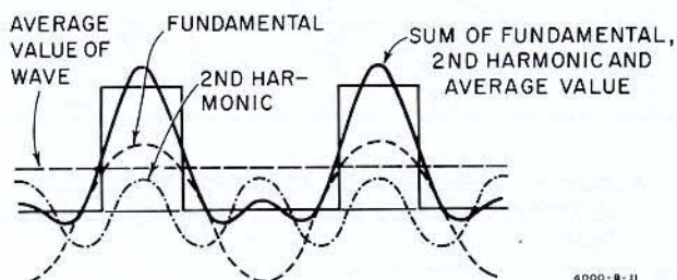
Figure 6b. Addition of a Fundamental Cosine Wave and its Harmonics to Form Rectangular Pulses
