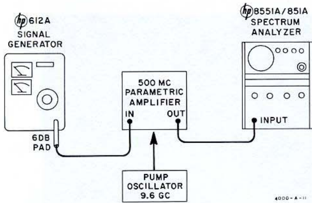
Figure 17. Parametric Amplifier Tuning Using Wide Spectrum Display of Analyzer
