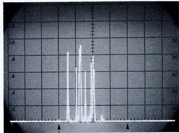
Figure 14. Appearance of a CW spectrum when analyzer's local oscillator has excessive FM.
