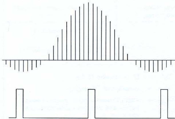
Figure 9a. Narrow pulse width causes wide spectrum lobes, high PRF results in low spectral line density.
