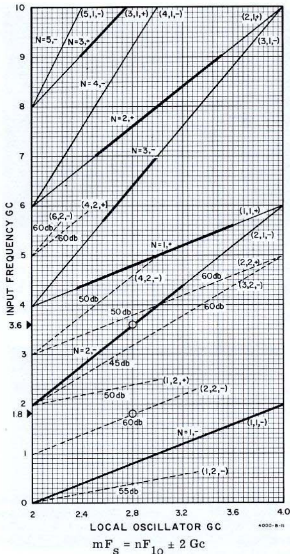
Figure 12c. \text{hp} Spectrum Analyzer Tuning Curves. Heavy solid lines indicate desired response locations for input signals of 10 Mc to 10 Gc. Spurious responses are indicated by the dashed lines.
