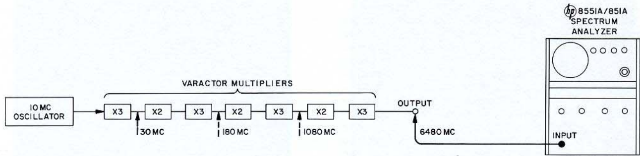
20 a. Test Setup for Varactor Multiplier Tuning
