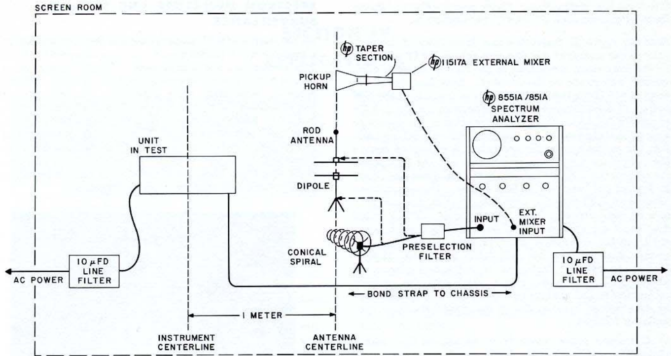
Figure 24. Suggested setup for measuring radiated RFI with the Spectrum Analyzer and appropriate antennas.
