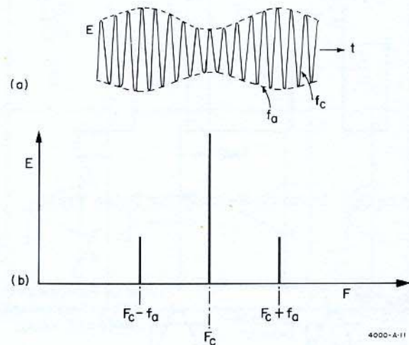
Figure 4. A Single Tone Amplitude Modulation, a) Time Amplitude Plot b) Frequency Amplitude Plot.
