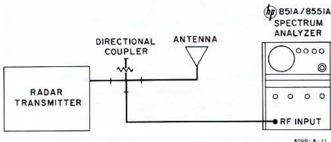
Figure 15. Spectrum Analyzer Connected for Checking Radar Magnetron Operation
