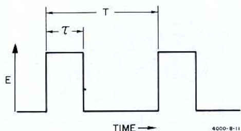
Figure 6a. Periodic Rectangular Pulse Train
