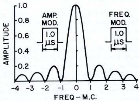
(a) Spectrum of rectangular pulse without AM or FM occurring during pulse. Shape is that of \frac{\sin \omega T/2}{\omega T/2} function.
