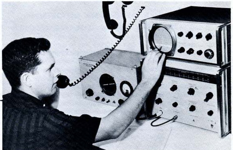
Figure 26. Broadband Spectrum Surveillance using \text{hp} Spectrum Analyzer. Operator monitors electromagnetic radiation in vicinity of launch area to ensure clear data channels and tracking frequencies.
