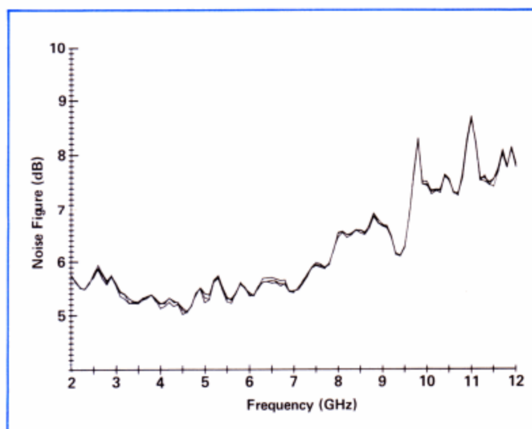
Figure 1-5. Three plots of the noise figure of a broadband receiver measured by three different sets of measuring equipment are within 0.1 dB at most frequencies.
