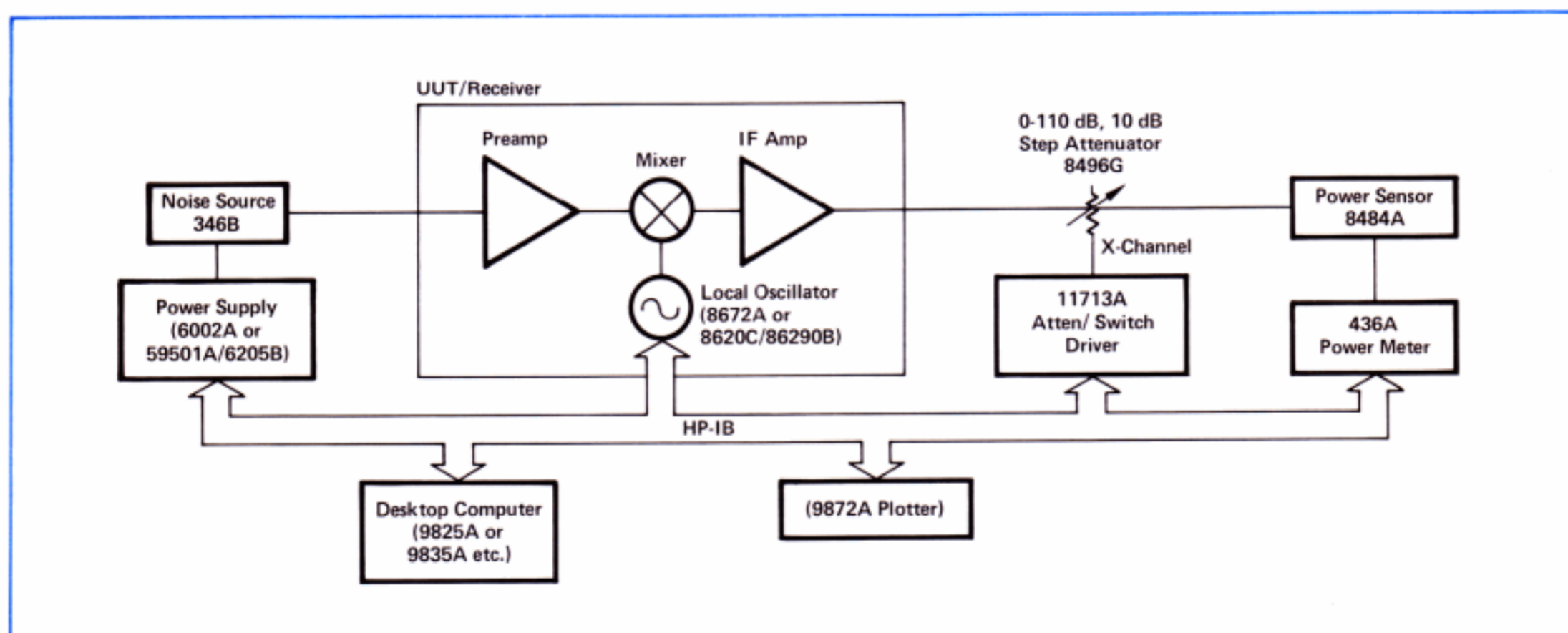
Figure 1-2. Block diagram of the general purpose noise figure measurement system. The unit under test can be all of or any part of the UUT/ Receiver portion of the block diagram. The remainder of the UUT/ Receiver block is then considered
