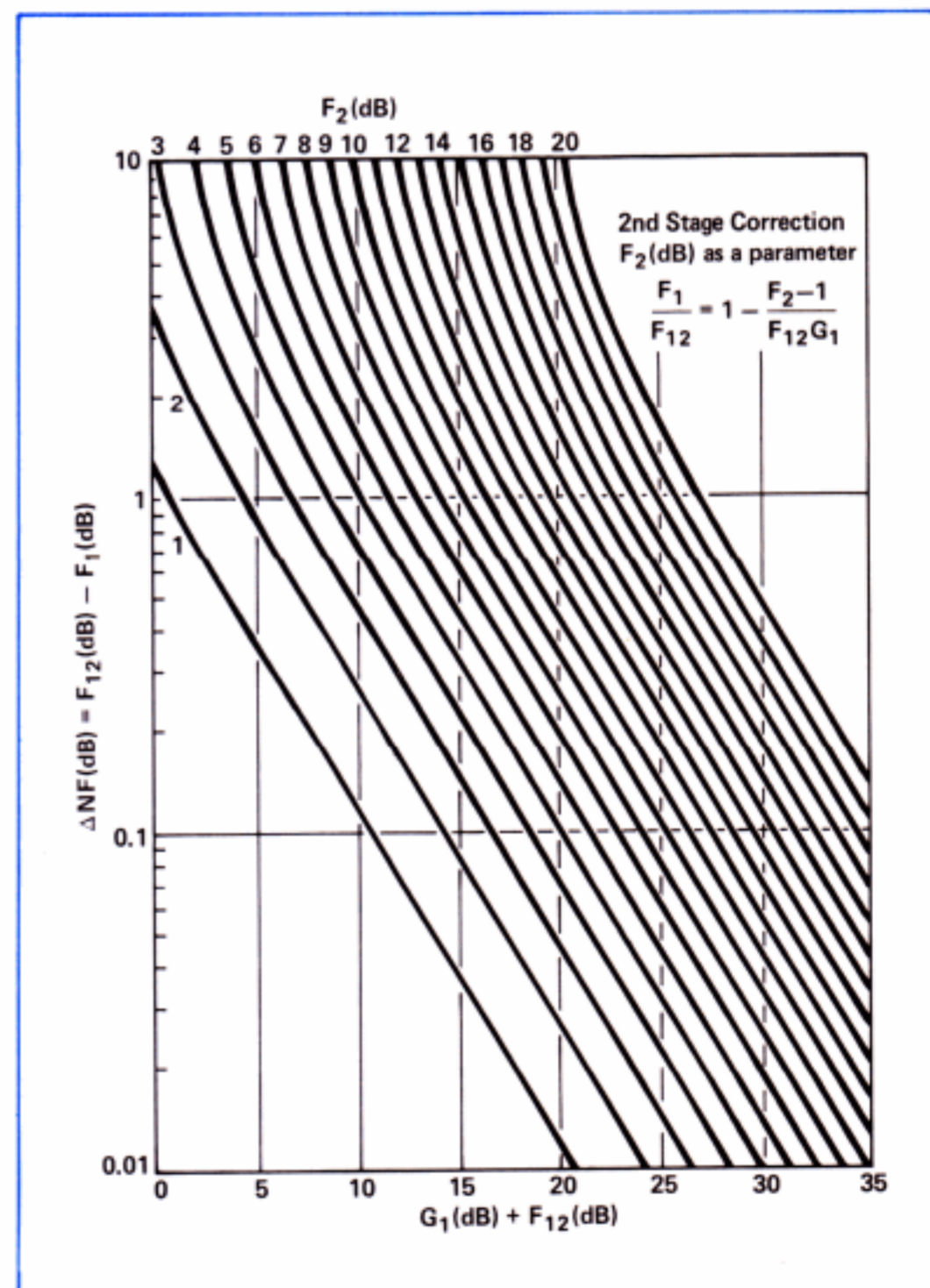
Figure 1-3. The correction due to the system's contribution of noise to measured data. After the calibration run, the computer performs this correction at each measurement frequency.
