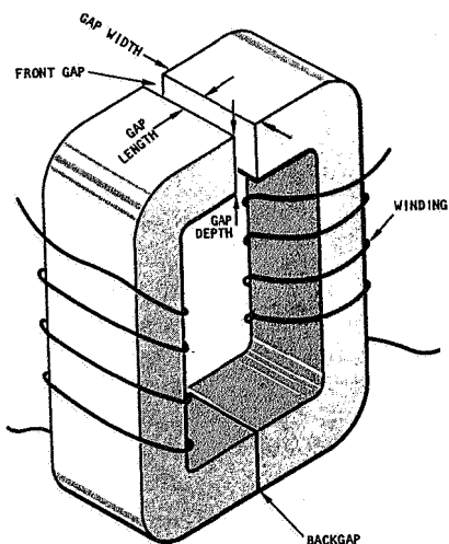
Figure 9. Head Core Showing Dimension Definitions
