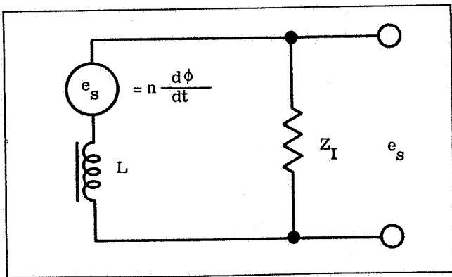
Figure 2. Voltage Equivalent Head Model
