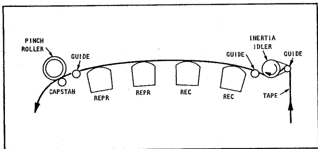
Figure 10. Open-Loop Drive
