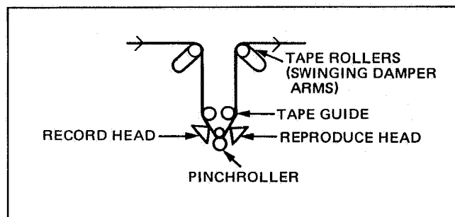
Figure 14. Refined Open-Loop Drive
