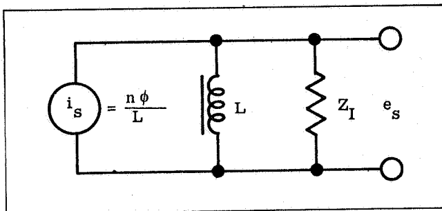
Figure 3. Current Equivalent Head Model
