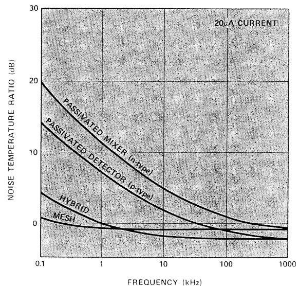
Figure 2. Typical Detector Noise
