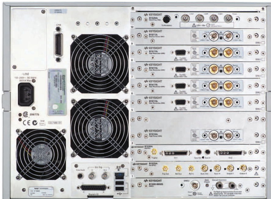
Figure 1. Wide choice of modules gives the B1500A great flexibility
