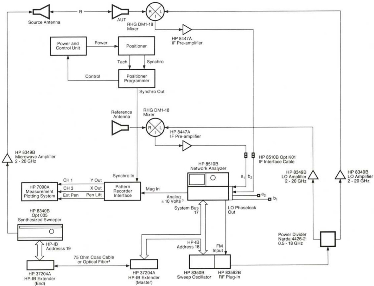
Figure 5. Detailed Hookup Diagram of External Phase-lock Configuration
