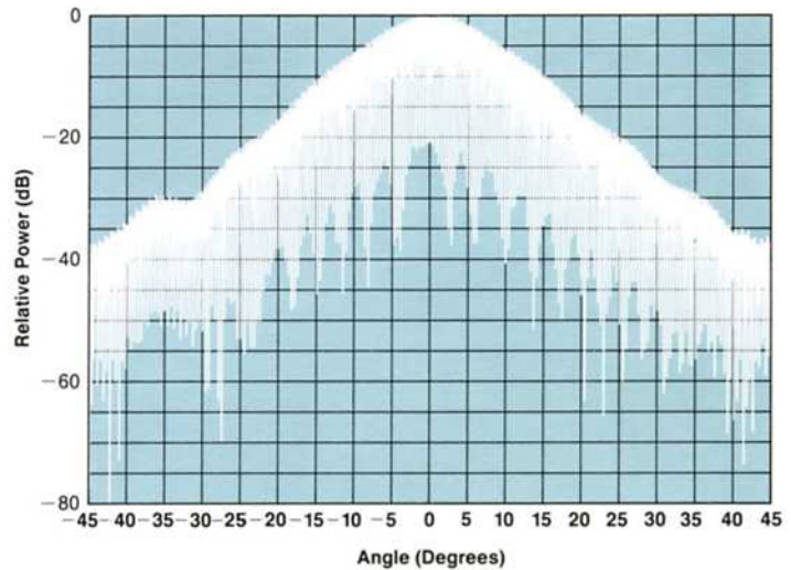
Figure 8. Rotating Source Polarization 80 dB Plot of X-band Standard Gain Horn at 10 GHz
