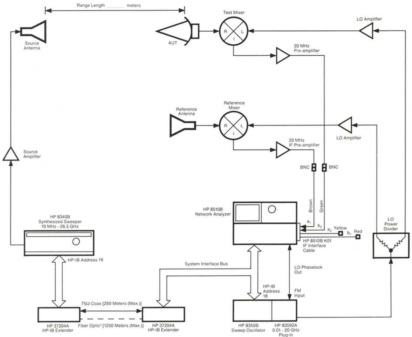
Figure 3. External Mixer Antenna Test System
