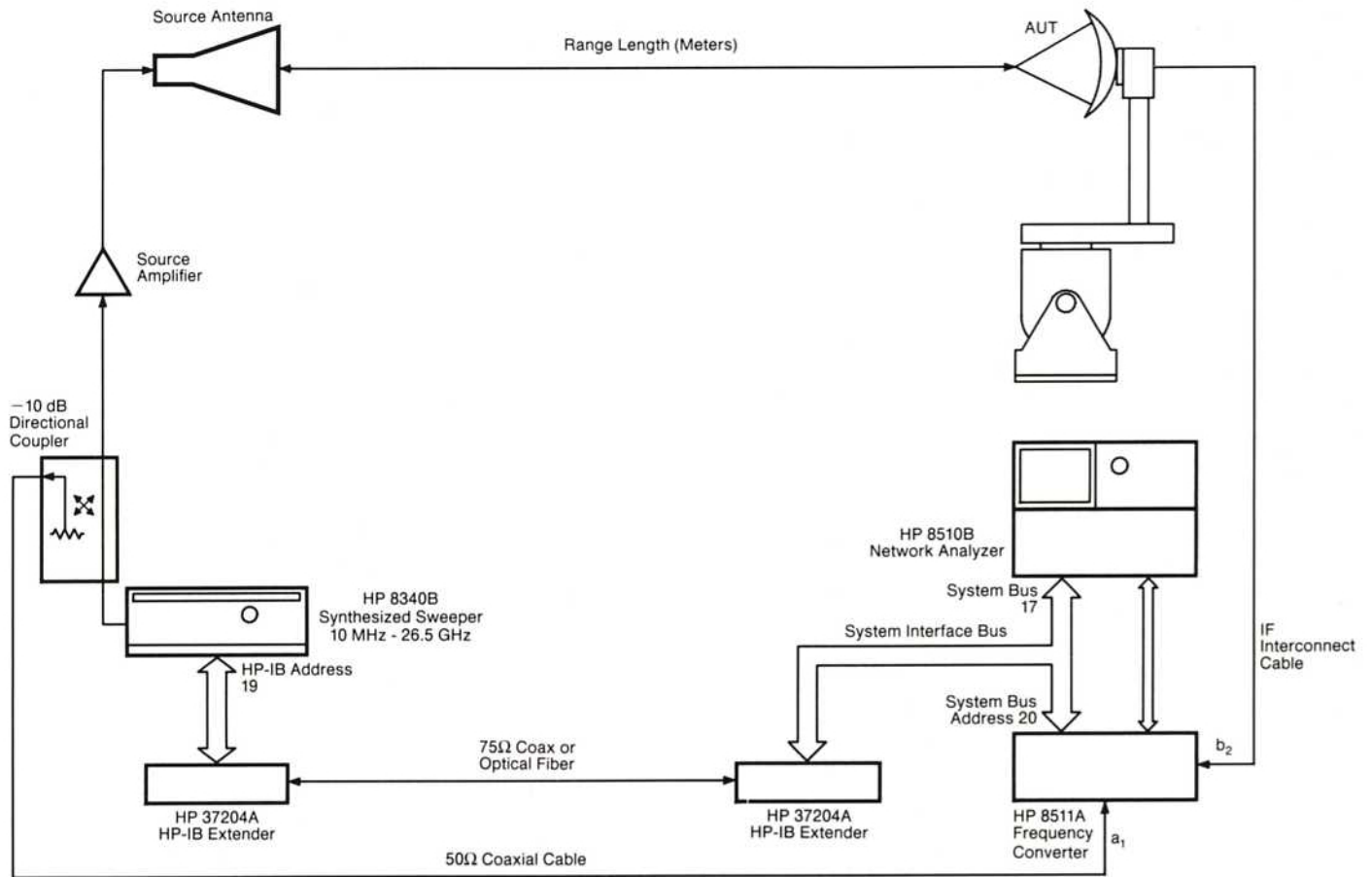
Figure 2. Antenna Test System Using an HP 8511A Frequency Converter
