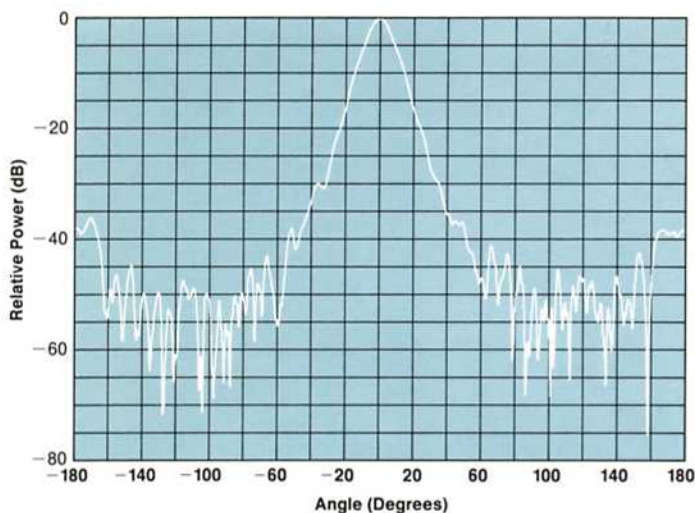
Figure 6. H-plane 80 dB Rectilinear Plot of a Standard Gain Horn at 10 GHz
