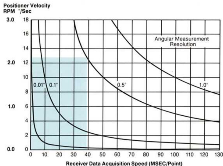
Figure 4. Positioner Velocity -vs- Acquisition Rate and Angular Resolution
