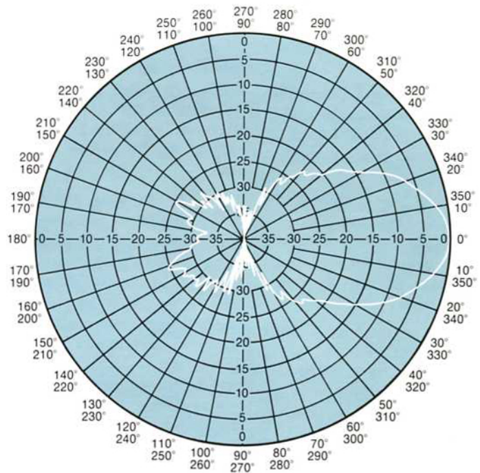
Figure 7. E-plane 40 dB Polar Plot of a Conical Broadband Horn at 8.5 GHz
