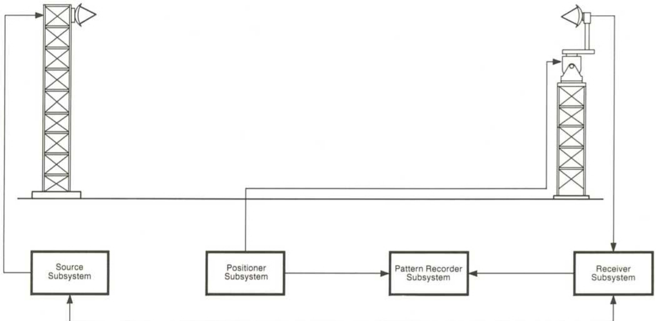
Figure 1. Typical Antenna Test System Block Diagram
