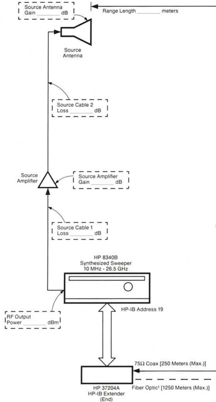
Figure A-2. Power Budget Worksheet for External Mixer Configuration
