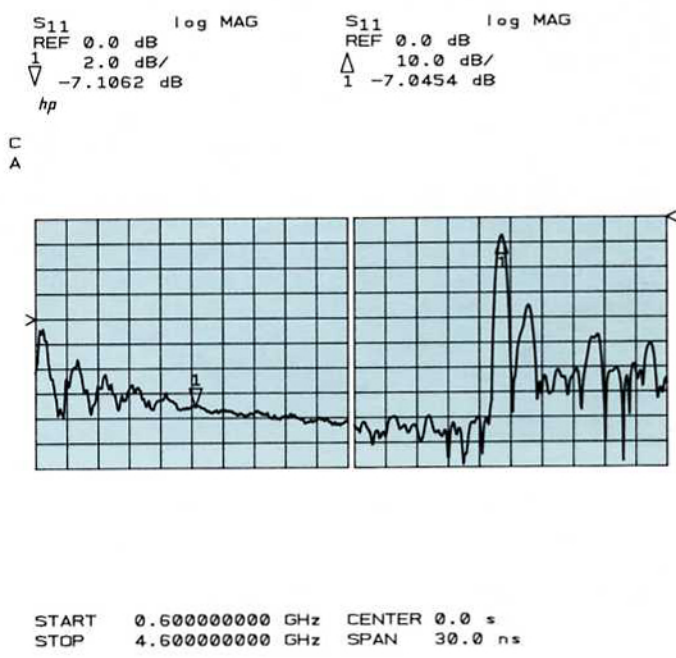
Figure 8. Calibrated RCS Frequency and Time Domain Responses of a Metal Sphere Using the 1-Port RCS Calibration Procedure.
