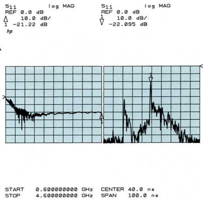
Figure 7. Uncalibrated RCS Frequency and Time Domain Responses of a Broadside Brass Cylinder.
