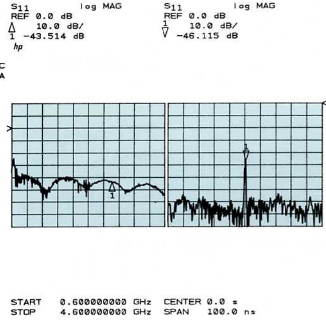
Figure 15. Calibrated RCS Frequency and Time Domain Responses of the Styrofoam Target.
