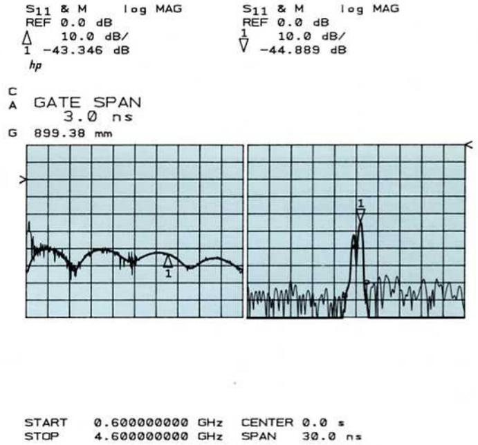
Figure 16. Gated RCS Frequency and Time Domain Responses of the Styrofoam Target.
