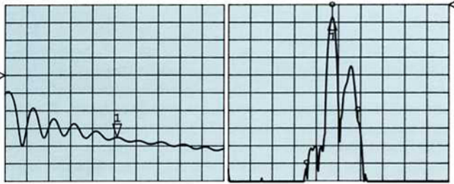
Figure 10. Effect of Reducing the Gate Span to Analyze the First Time Domain Response of the Sphere.
