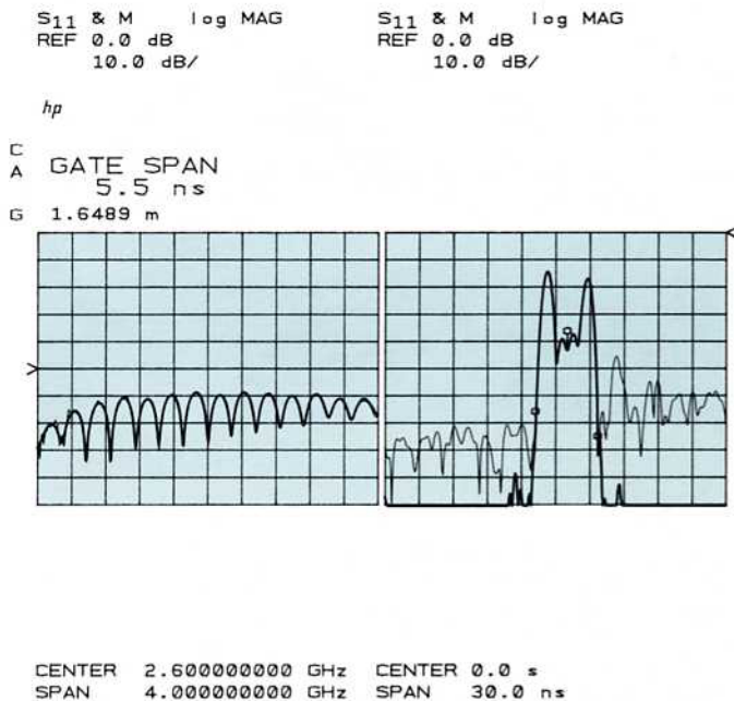
Figure 13. Gated and Ungated RCS Responses of the Brass Cylinder Turned End-on with the Metal Sphere Used as Reference.
