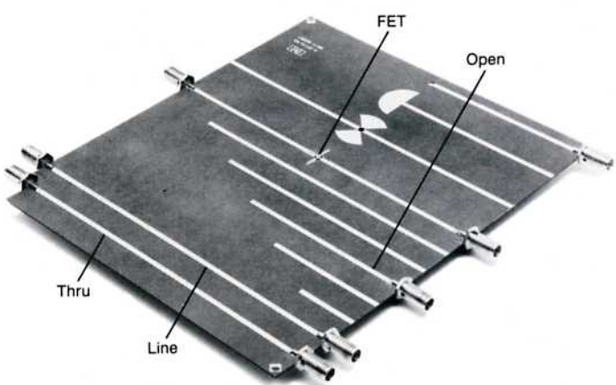
Figure 15. Microstrip PC board as a test fixture including separate transmission lines as the THRU and LINE, an open circuit and a test line for insertion of a test device.
