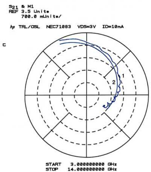
Figure 16. Example measurement of a linear FET on the microstrip PC board compared to measurement in a de-embedded test fixture (HP 85041A). (1) de-embedded measurement (2) TRL calibration using PC board standards.
