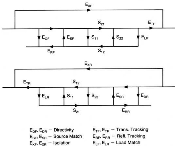
Figure 3. Two-port 12-term error model.
