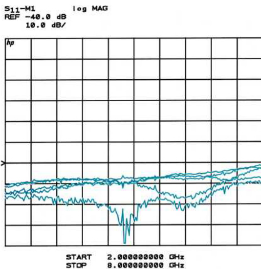
Figure 19. Connection repeatability of the microstrip test fixture.
