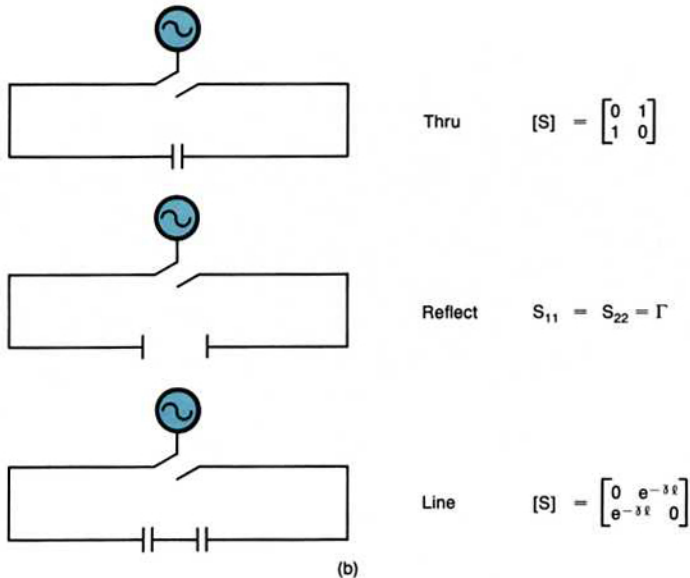
Figure 6. (a) 8-term TRL error model and generalized coefficients. (b) TRL procedure and assumed S-parameter values for each step.
