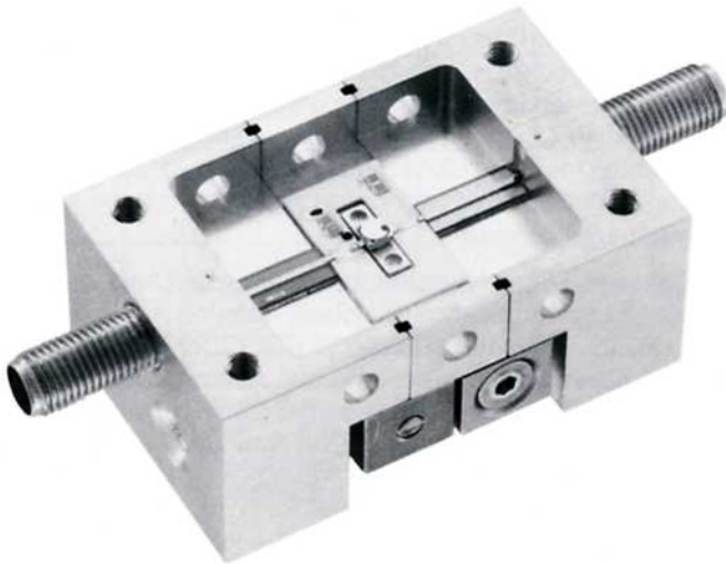
Figure 1. Microstrip test fixture.
