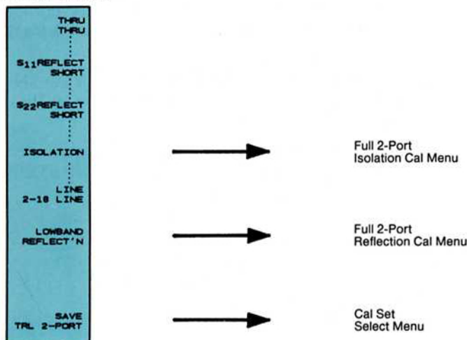
Figure 18. TRL 2-PORT calibration menu.
