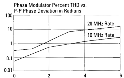
Figure 3. Phase modulator distortion
