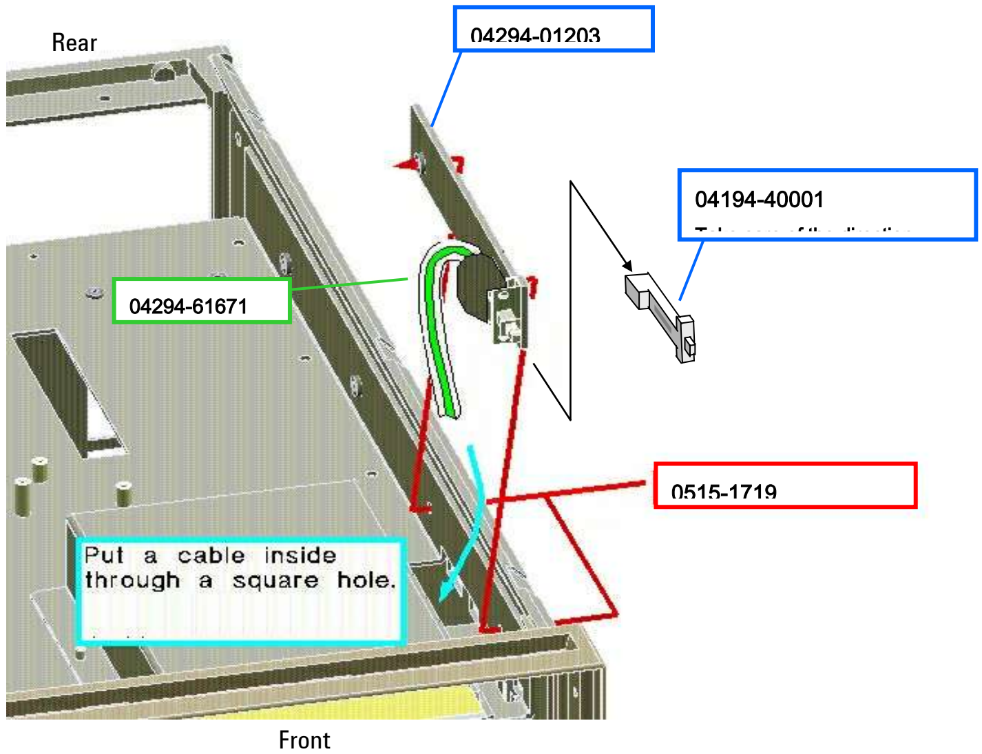
Figure 1 Replaceable Parts from Bottom View
