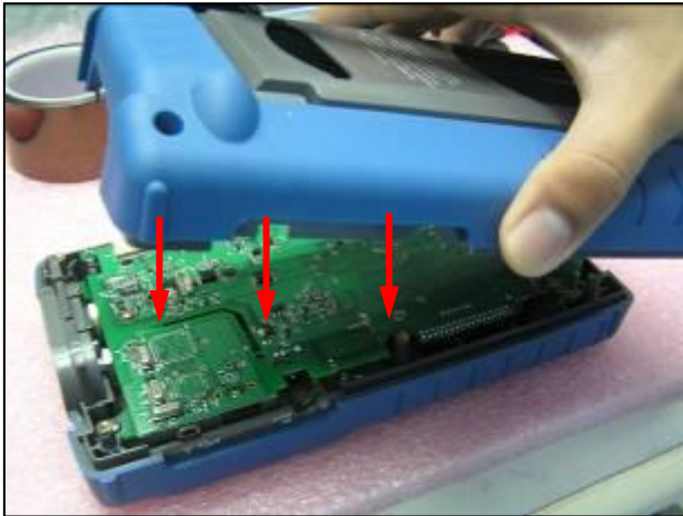
Figure 11 Put the rear housing back
