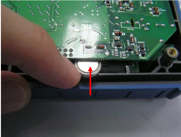
Figure 10 Push the button cell into the holder
