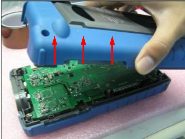
Figure 6 Remove the rear casing from the instrument
