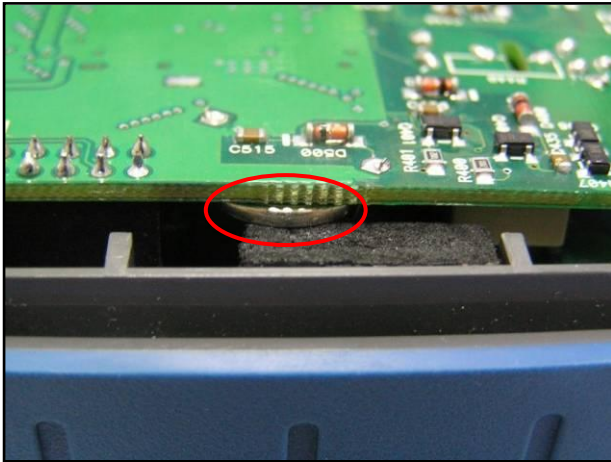
Figure 7 Button cell at the left edge of the PCB
