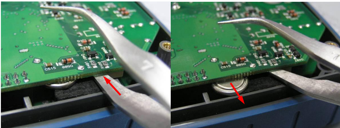
Figure 9 Push the button cell out from the holder
